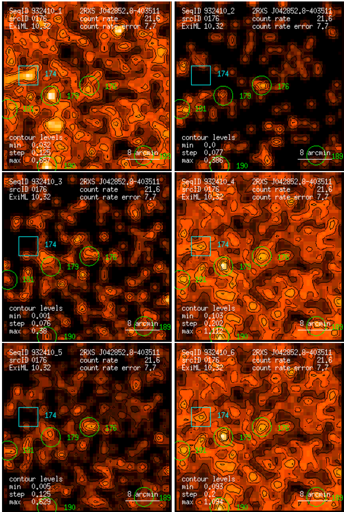
Figure 176: RASS 932410: detection 0176: band rate images, Gaussian filter: (1) PSPC channels 11 – 41, (2) 52 – 90, (3) 91 – 201, (4) 11 – 235, (5) 52 – 201, (6) 11 – 201. Broad band rates in counts/ks. Band rate contour levels in counts/ks/arcmin 2 .
