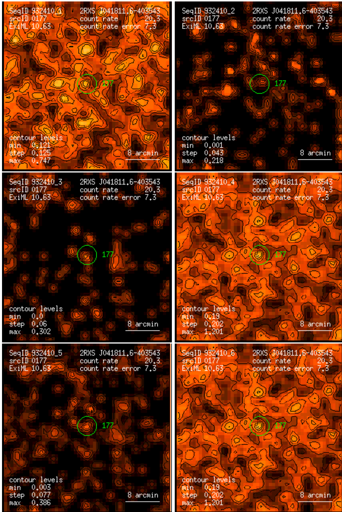
Figure 177: RASS 932410: detection 0177: band rate images, Gaussian filter: (1) PSPC channels 11 – 41, (2) 52 – 90, (3) 91 – 201, (4) 11 – 235, (5) 52 – 201, (6) 11 – 201. Broad band rates in counts/ks. Band rate contour levels in counts/ks/arcmin 2 .
