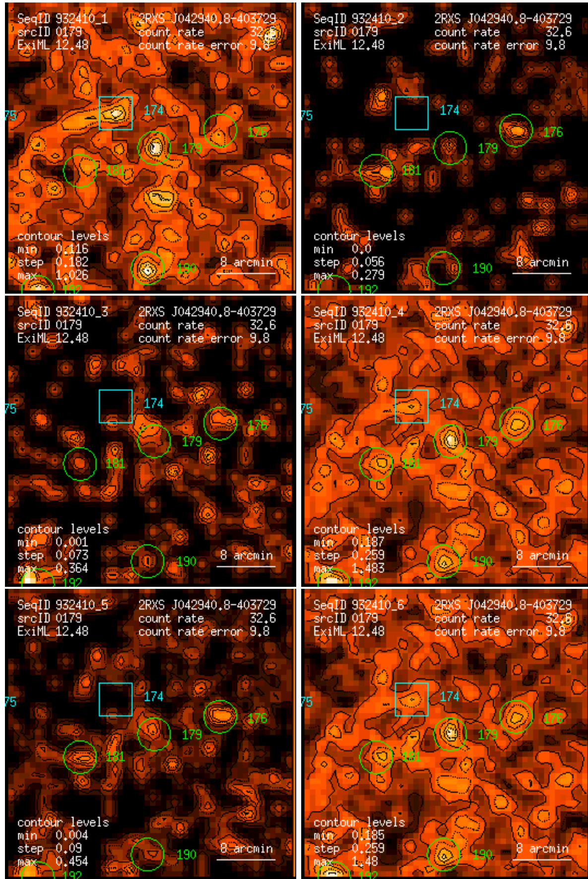
Figure 179: RASS 932410: detection 0179: band rate images, Gaussian filter: (1) PSPC channels 11 – 41, (2) 52 – 90, (3) 91 – 201, (4) 11 – 235, (5) 52 – 201, (6) 11 – 201. Broad band rates in counts/ks. Band rate contour levels in counts/ks/arcmin 2 .
