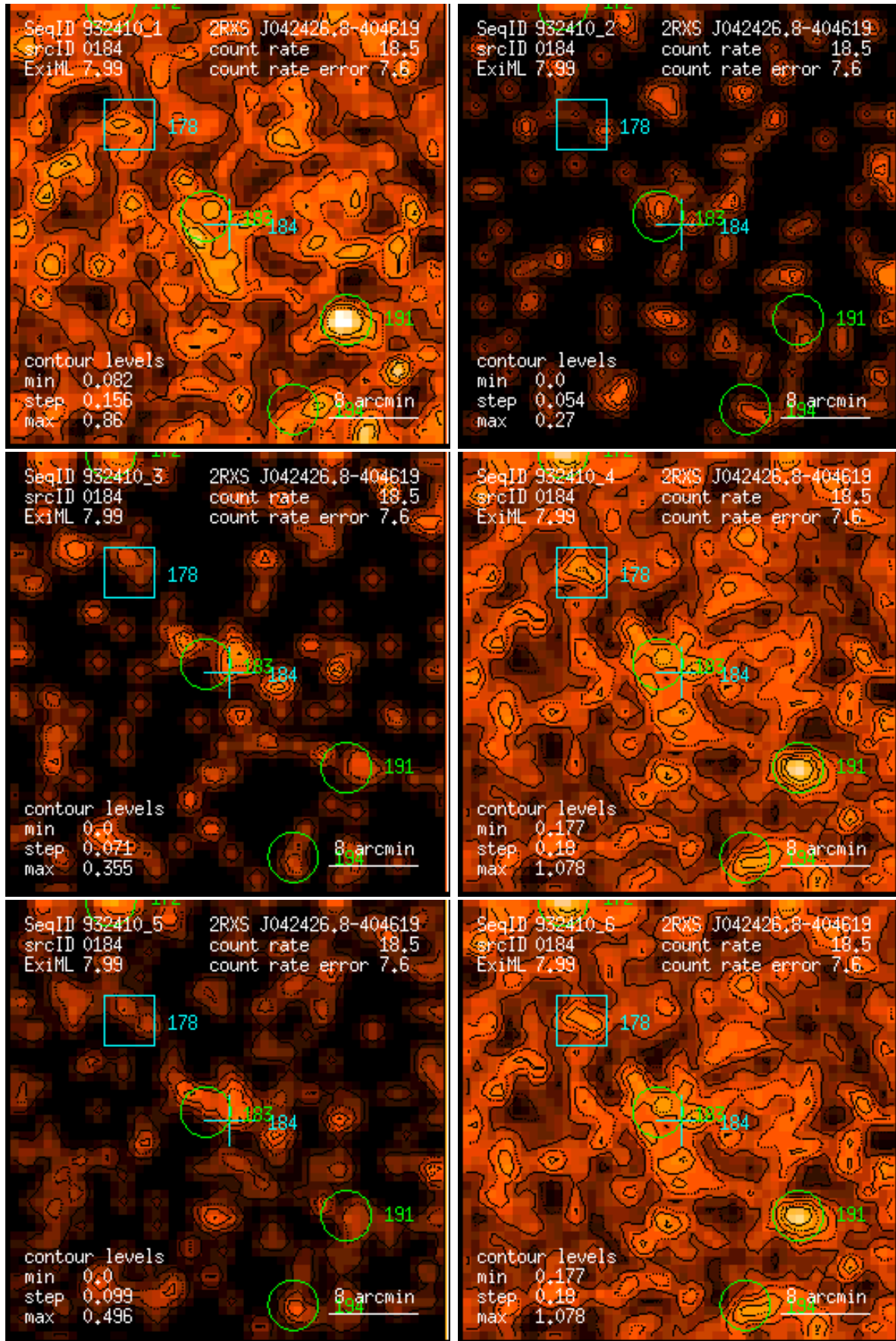
Figure 184: RASS 932410: detection 0184: band rate images, Gaussian filter: (1) PSPC channels 11 – 41, (2) 52 – 90, (3) 91 – 201, (4) 11 – 235, (5) 52 – 201, (6) 11 – 201. Broad band rates in counts/ks. Band rate contour levels in counts/ks/arcmin 2 .
