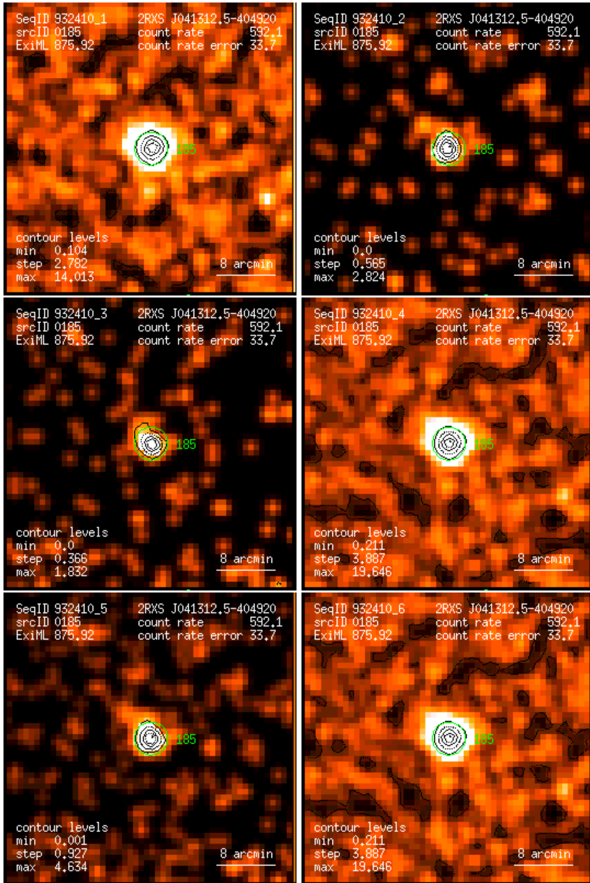
Figure 185: RASS 932410: detection 0185: band rate images, Gaussian filter: (1) PSPC channels 11 – 41, (2) 52 – 90, (3) 91 – 201, (4) 11 – 235, (5) 52 – 201, (6) 11 – 201. Broad band rates in counts/ks. Band rate contour levels in counts/ks/arcmin 2 .
