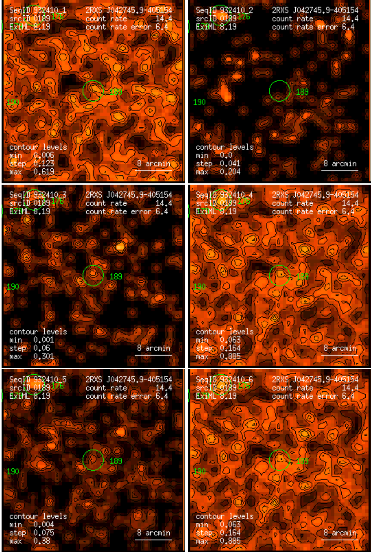
Figure 189: RASS 932410: detection 0189: band rate images, Gaussian filter: (1) PSPC channels 11 – 41, (2) 52 – 90, (3) 91 – 201, (4) 11 – 235, (5) 52 – 201, (6) 11 – 201. Broad band rates in counts/ks. Band rate contour levels in counts/ks/arcmin 2 .
