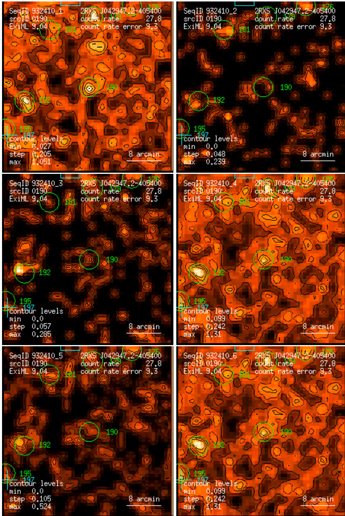
Figure 190: RASS 932410: detection 0190: band rate images, Gaussian filter: (1) PSPC channels 11 – 41, (2) 52 – 90, (3) 91 – 201, (4) 11 – 235, (5) 52 – 201, (6) 11 – 201. Broad band rates in counts/ks. Band rate contour levels in counts/ks/arcmin 2 .
