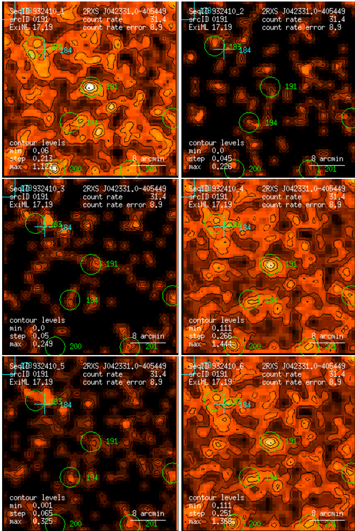
Figure 191: RASS 932410: detection 0191: band rate images, Gaussian filter: (1) PSPC channels 11 – 41, (2) 52 – 90, (3) 91 – 201, (4) 11 – 235, (5) 52 – 201, (6) 11 – 201. Broad band rates in counts/ks. Band rate contour levels in counts/ks/arcmin 2 .
