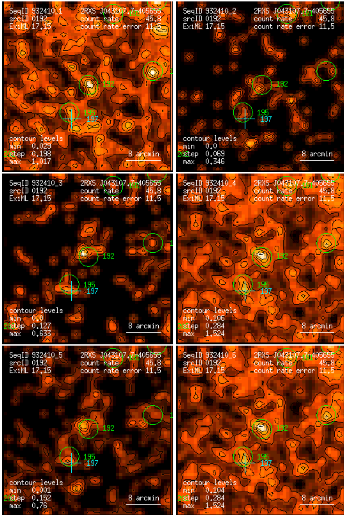
Figure 192: RASS 932410: detection 0192: band rate images, Gaussian filter: (1) PSPC channels 11 – 41, (2) 52 – 90, (3) 91 – 201, (4) 11 – 235, (5) 52 – 201, (6) 11 – 201. Broad band rates in counts/ks. Band rate contour levels in counts/ks/arcmin 2 .
