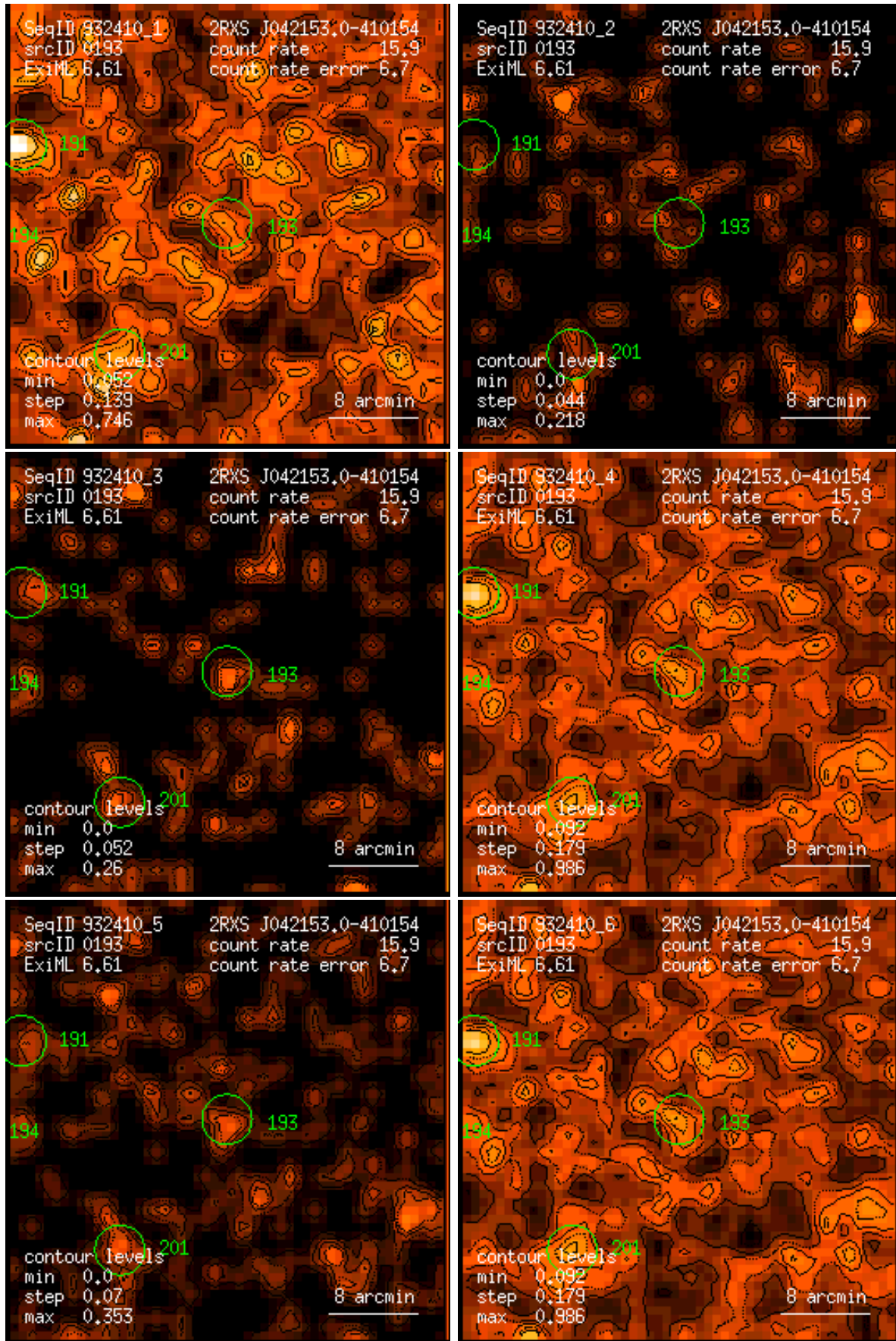
Figure 193: RASS 932410: detection 0193: band rate images, Gaussian filter: (1) PSPC channels 11 – 41, (2) 52 – 90, (3) 91 – 201, (4) 11 – 235, (5) 52 – 201, (6) 11 – 201. Broad band rates in counts/ks. Band rate contour levels in counts/ks/arcmin 2 .
