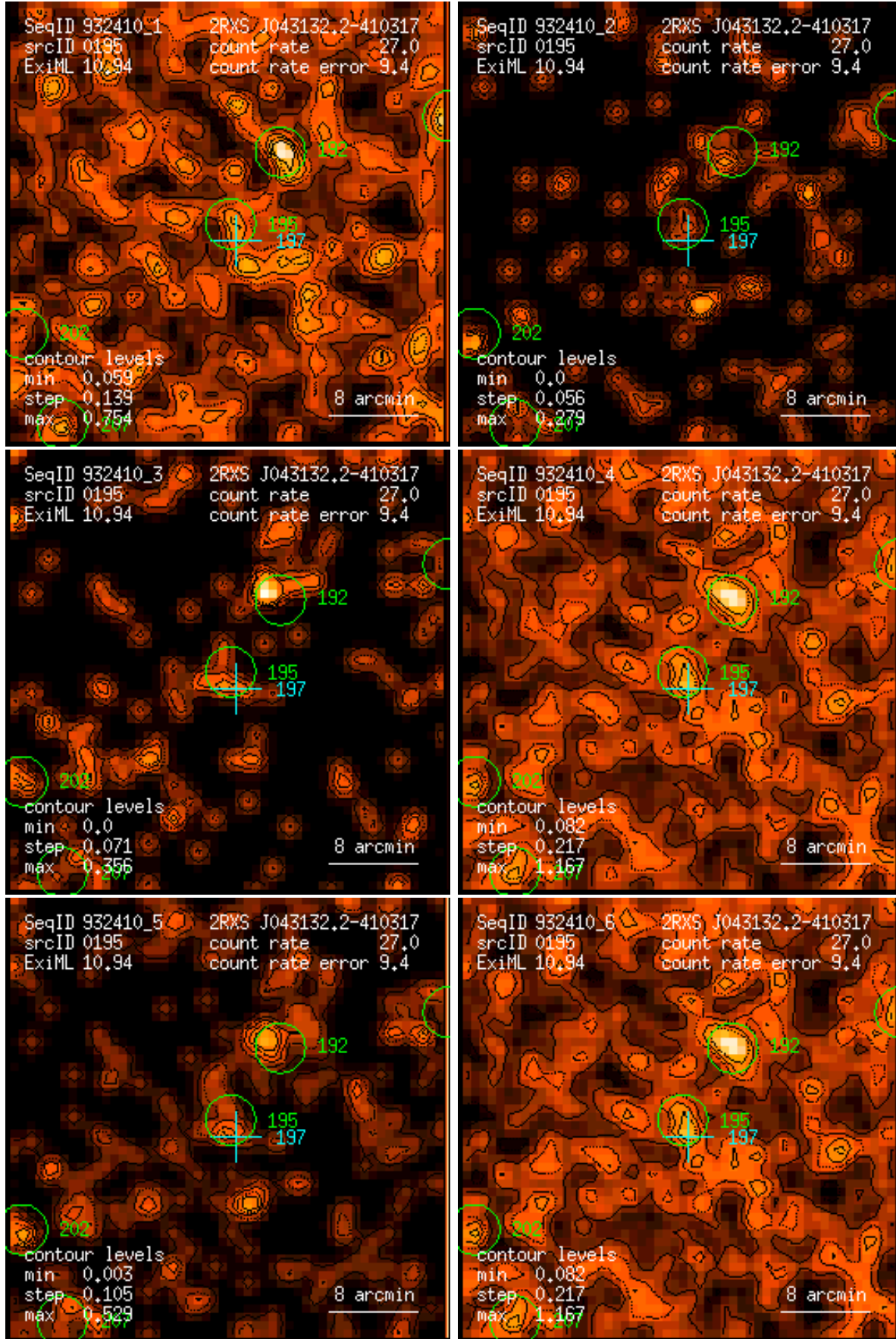
Figure 195: RASS 932410: detection 0195: band rate images, Gaussian filter: (1) PSPC channels 11 – 41, (2) 52 – 90, (3) 91 – 201, (4) 11 – 235, (5) 52 – 201, (6) 11 – 201. Broad band rates in counts/ks. Band rate contour levels in counts/ks/arcmin 2 .
