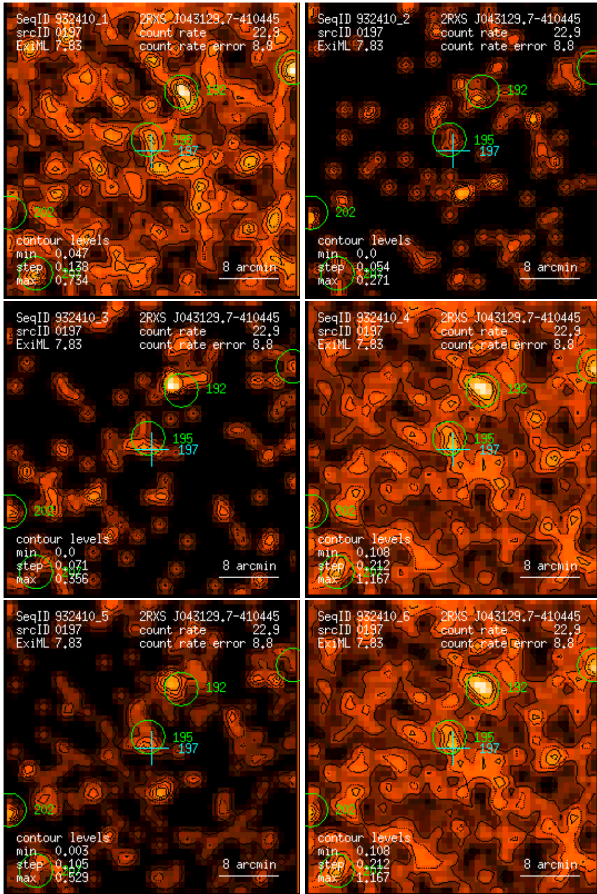
Figure 197: RASS 932410: detection 0197: band rate images, Gaussian filter: (1) PSPC channels 11 – 41, (2) 52 – 90, (3) 91 – 201, (4) 11 – 235, (5) 52 – 201, (6) 11 – 201. Broad band rates in counts/ks. Band rate contour levels in counts/ks/arcmin 2 .
