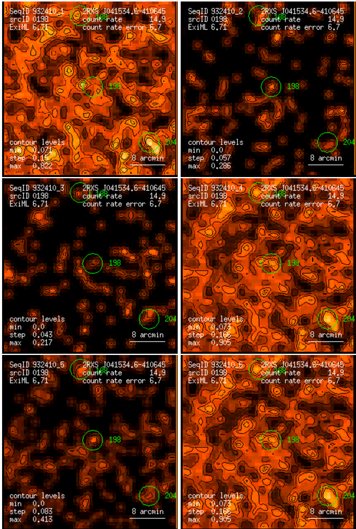
Figure 198: RASS 932410: detection 0198: band rate images, Gaussian filter: (1) PSPC channels 11 – 41, (2) 52 – 90, (3) 91 – 201, (4) 11 – 235, (5) 52 – 201, (6) 11 – 201. Broad band rates in counts/ks. Band rate contour levels in counts/ks/arcmin 2 .
