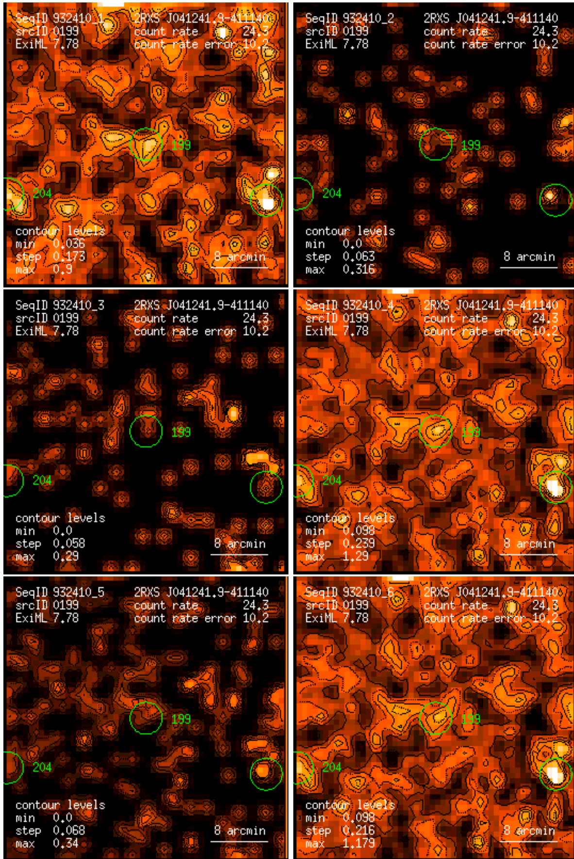
Figure 199: RASS 932410: detection 0199: band rate images, Gaussian filter: (1) PSPC channels 11 – 41, (2) 52 – 90, (3) 91 – 201, (4) 11 – 235, (5) 52 – 201, (6) 11 – 201. Broad band rates in counts/ks. Band rate contour levels in counts/ks/arcmin 2 .
