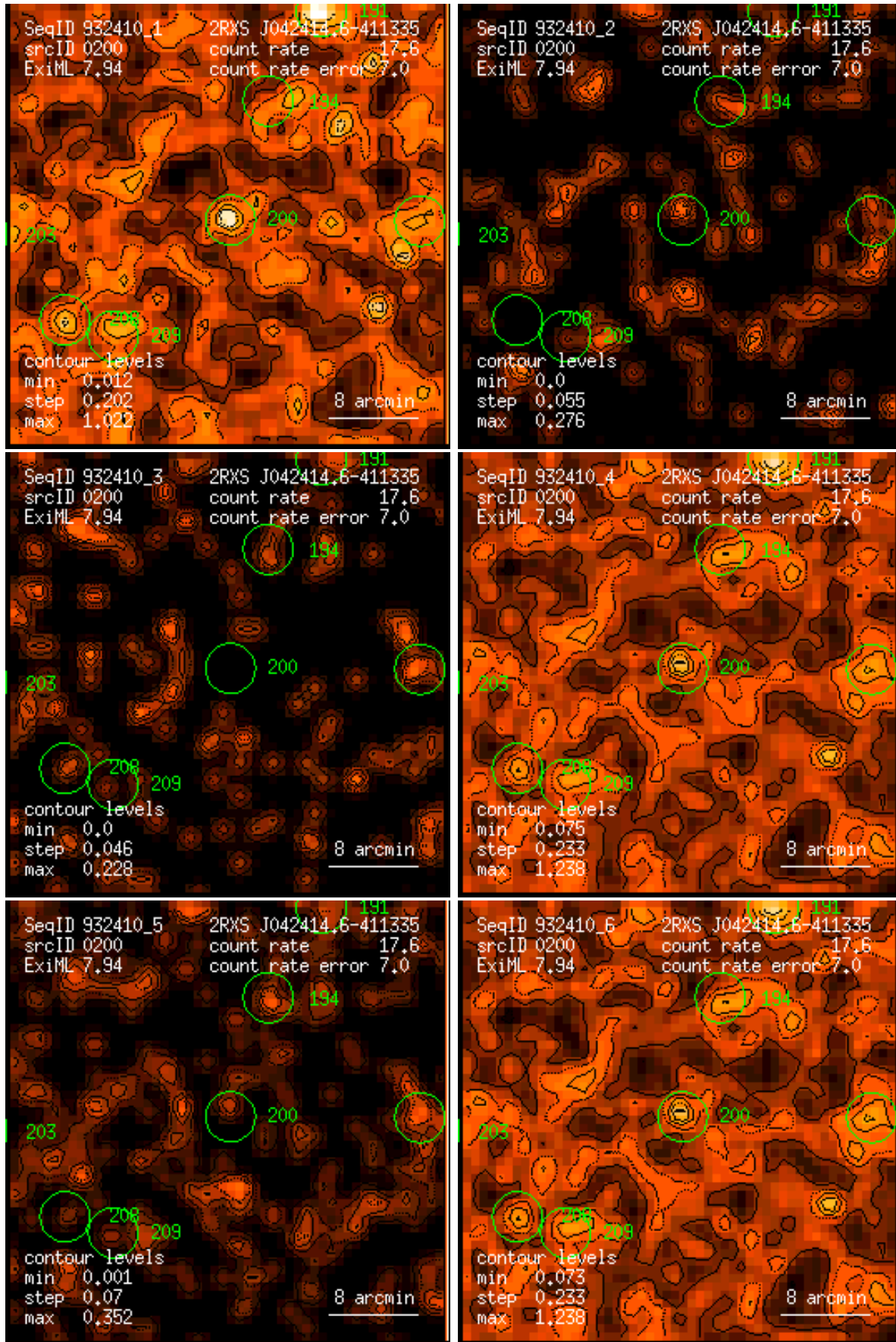
Figure 200: RASS 932410: detection 0200: band rate images, Gaussian filter: (1) PSPC channels 11 – 41, (2) 52 – 90, (3) 91 – 201, (4) 11 – 235, (5) 52 – 201, (6) 11 – 201. Broad band rates in counts/ks. Band rate contour levels in counts/ks/arcmin 2 .
