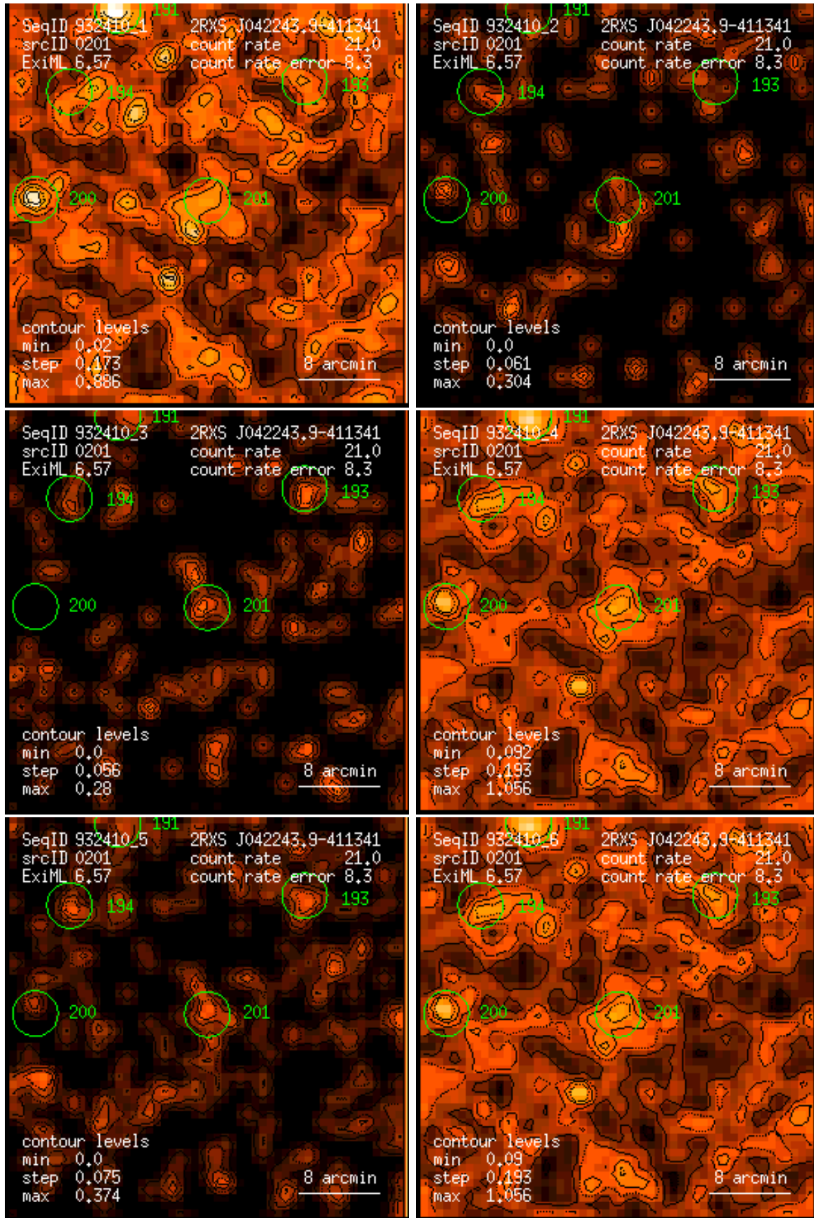
Figure 201: RASS 932410: detection 0201: band rate images, Gaussian filter: (1) PSPC channels 11 – 41, (2) 52 – 90, (3) 91 – 201, (4) 11 – 235, (5) 52 – 201, (6) 11 – 201. Broad band rates in counts/ks. Band rate contour levels in counts/ks/arcmin 2 .
