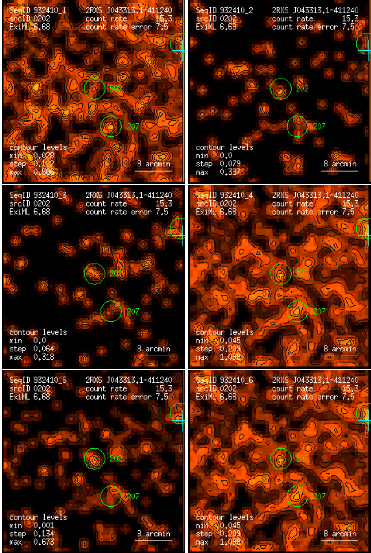
Figure 202: RASS 932410: detection 0202: band rate images, Gaussian filter: (1) PSPC channels 11 – 41, (2) 52 – 90, (3) 91 – 201, (4) 11 – 235, (5) 52 – 201, (6) 11 – 201. Broad band rates in counts/ks. Band rate contour levels in counts/ks/arcmin 2 .
