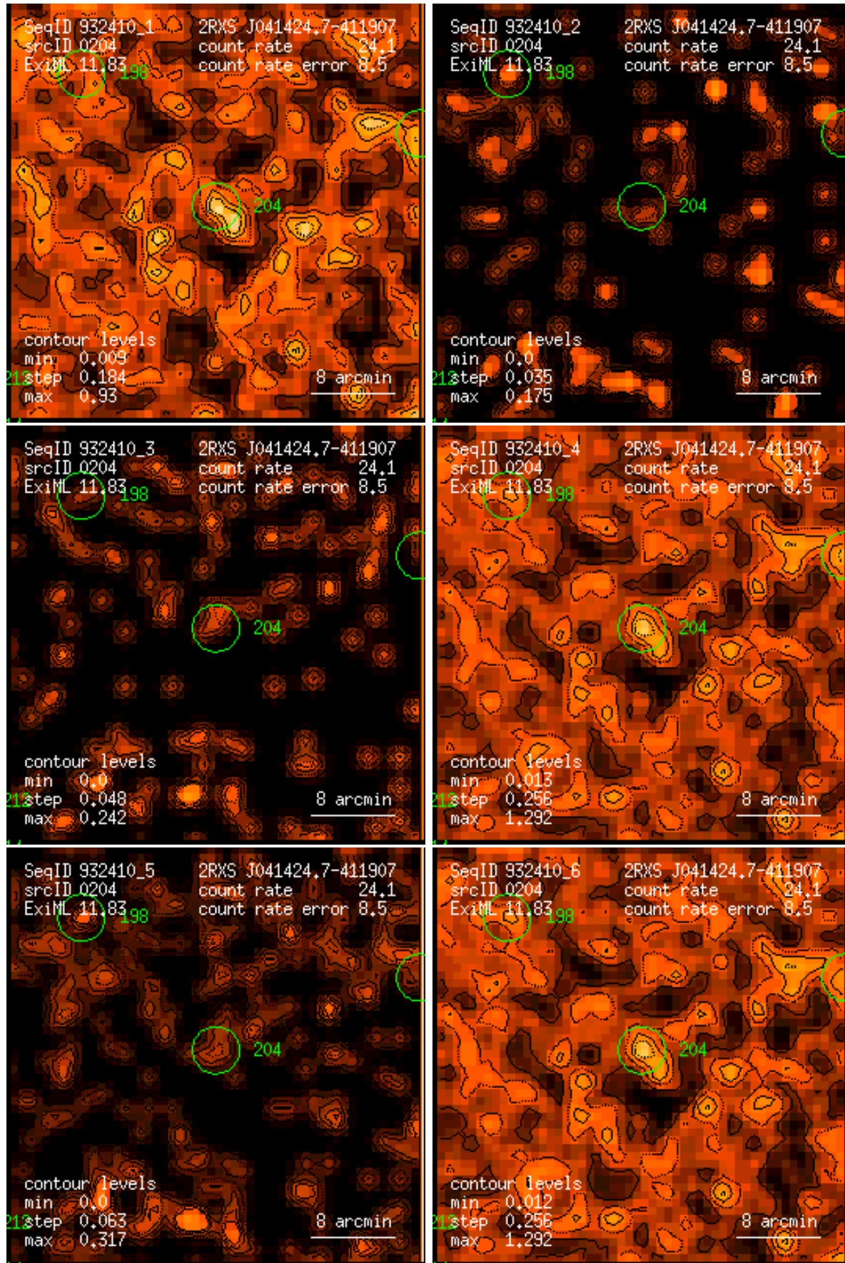
Figure 204: RASS 932410: detection 0204: band rate images, Gaussian filter: (1) PSPC channels 11 – 41, (2) 52 – 90, (3) 91 – 201, (4) 11 – 235, (5) 52 – 201, (6) 11 – 201. Broad band rates in counts/ks. Band rate contour levels in counts/ks/arcmin 2 .
