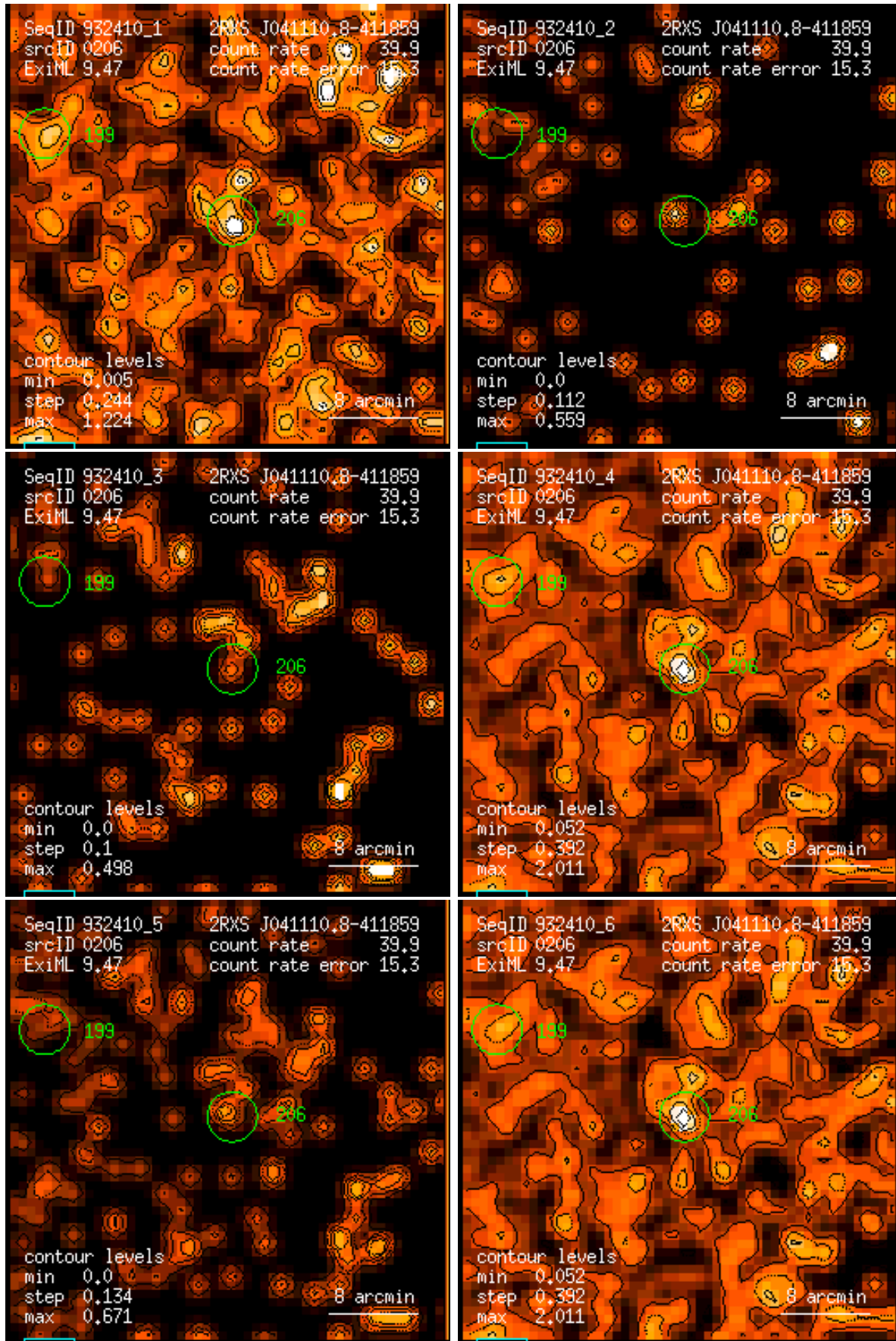
Figure 206: RASS 932410: detection 0206: band rate images, Gaussian filter: (1) PSPC channels 11 – 41, (2) 52 – 90, (3) 91 – 201, (4) 11 – 235, (5) 52 – 201, (6) 11 – 201. Broad band rates in counts/ks. Band rate contour levels in counts/ks/arcmin 2 .
