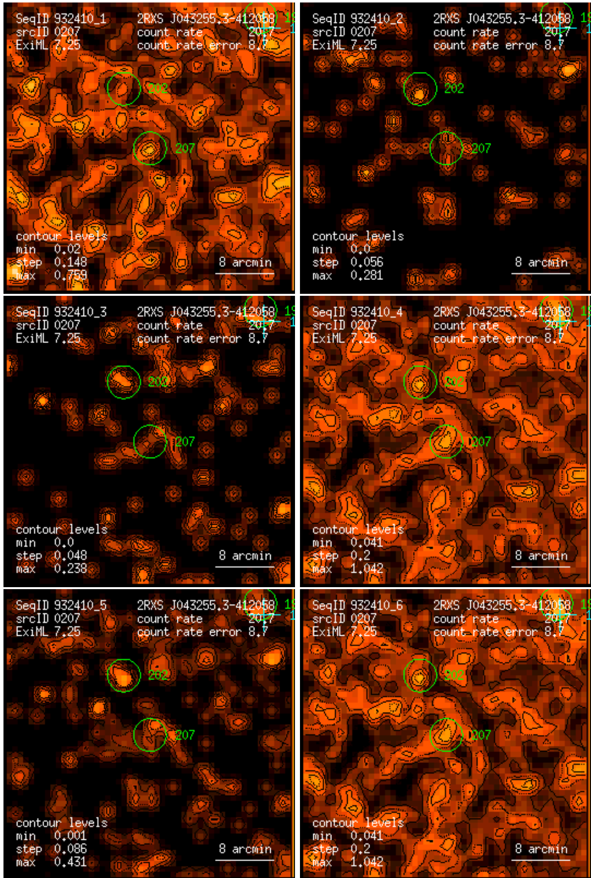
Figure 207: RASS 932410: detection 0207: band rate images, Gaussian filter: (1) PSPC channels 11 – 41, (2) 52 – 90, (3) 91 – 201, (4) 11 – 235, (5) 52 – 201, (6) 11 – 201. Broad band rates in counts/ks. Band rate contour levels in counts/ks/arcmin 2 .
