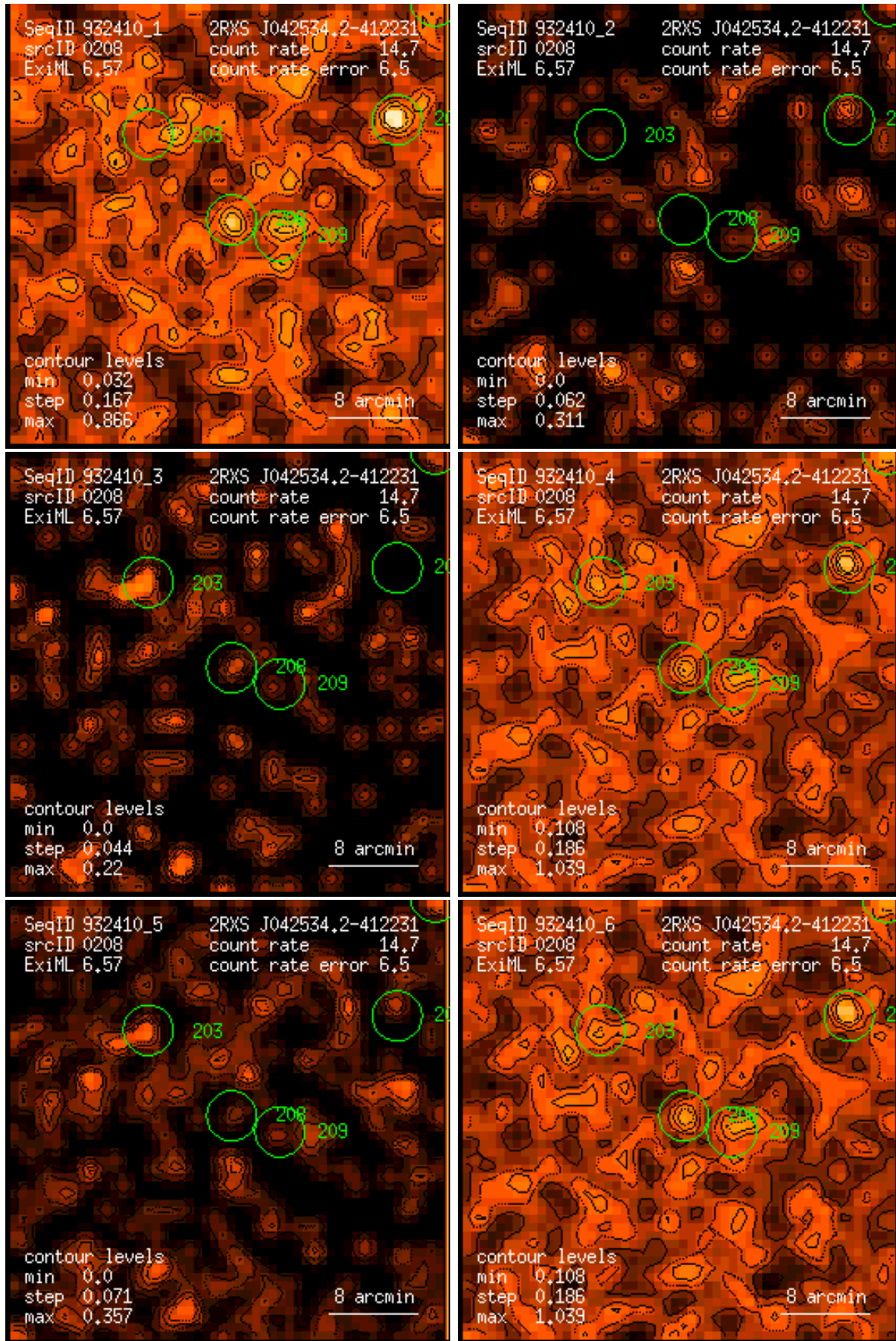
Figure 208: RASS 932410: detection 0208: band rate images, Gaussian filter: (1) PSPC channels 11 – 41, (2) 52 – 90, (3) 91 – 201, (4) 11 – 235, (5) 52 – 201, (6) 11 – 201. Broad band rates in counts/ks. Band rate contour levels in counts/ks/arcmin 2 .
