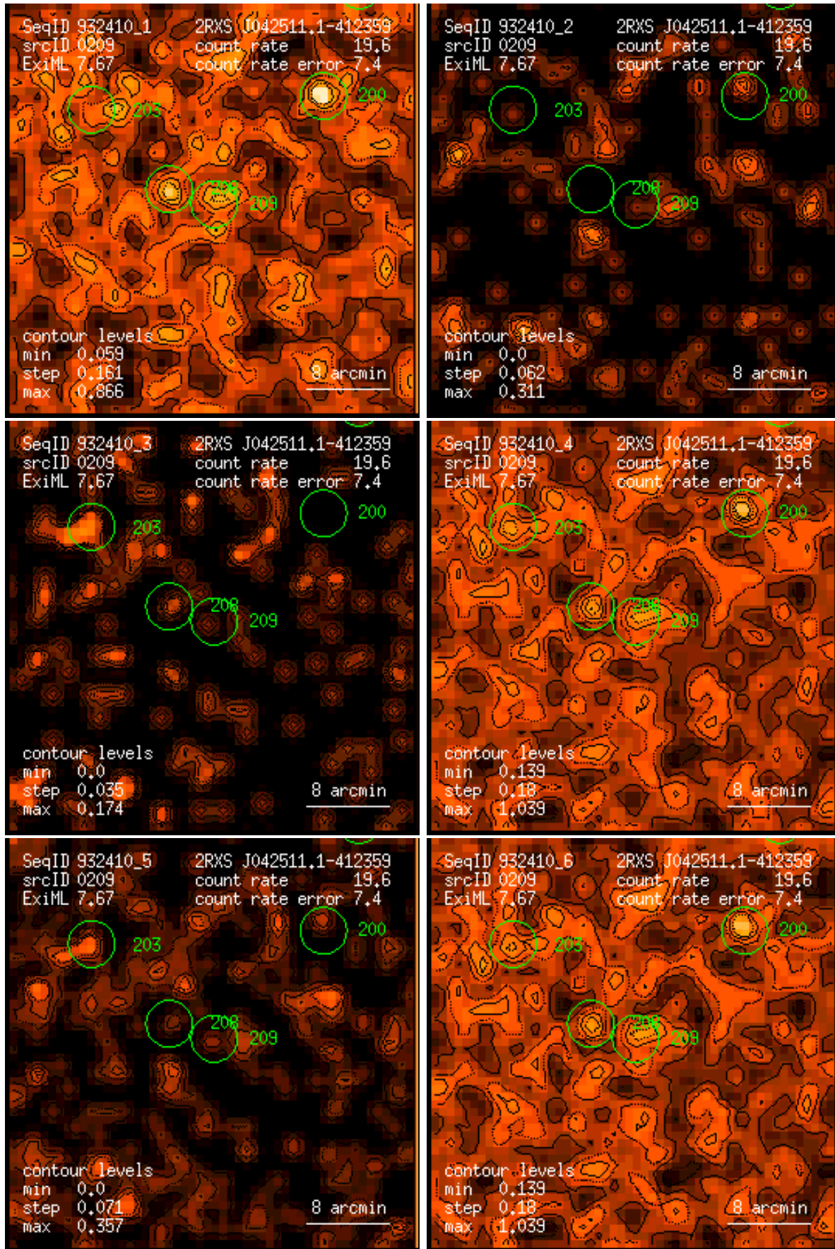
Figure 209: RASS 932410: detection 0209: band rate images, Gaussian filter: (1) PSPC channels 11 – 41, (2) 52 – 90, (3) 91 – 201, (4) 11 – 235, (5) 52 – 201, (6) 11 – 201. Broad band rates in counts/ks. Band rate contour levels in counts/ks/arcmin 2 .
