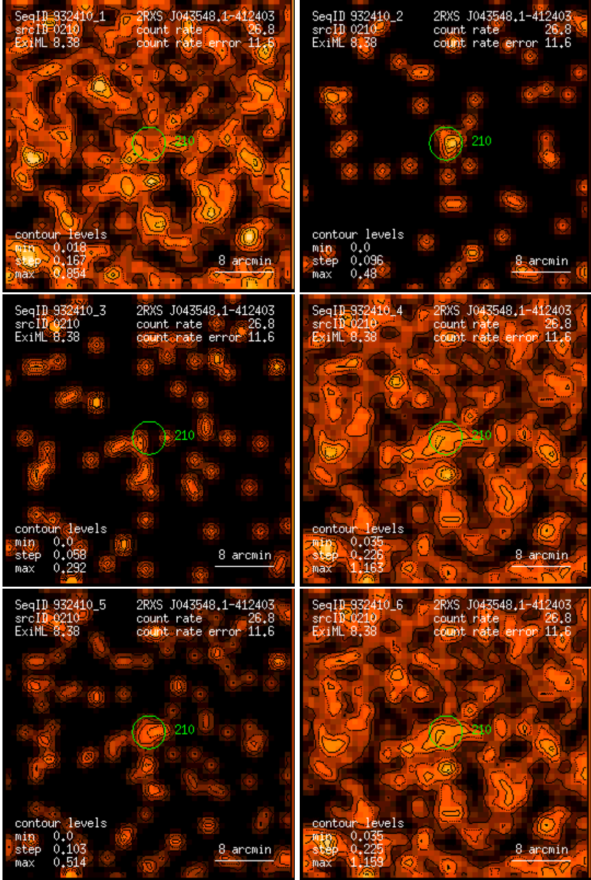
Figure 210: RASS 932410: detection 0210: band rate images, Gaussian filter: (1) PSPC channels 11 – 41, (2) 52 – 90, (3) 91 – 201, (4) 11 – 235, (5) 52 – 201, (6) 11 – 201. Broad band rates in counts/ks. Band rate contour levels in counts/ks/arcmin 2 .
