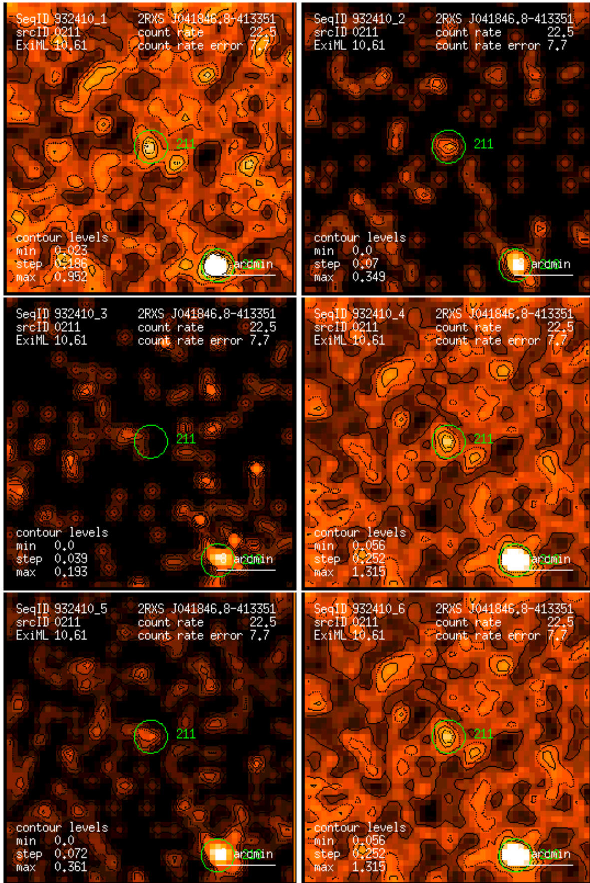
Figure 211: RASS 932410: detection 0211: band rate images, Gaussian filter: (1) PSPC channels 11 – 41, (2) 52 – 90, (3) 91 – 201, (4) 11 – 235, (5) 52 – 201, (6) 11 – 201. Broad band rates in counts/ks. Band rate contour levels in counts/ks/arcmin 2 .
