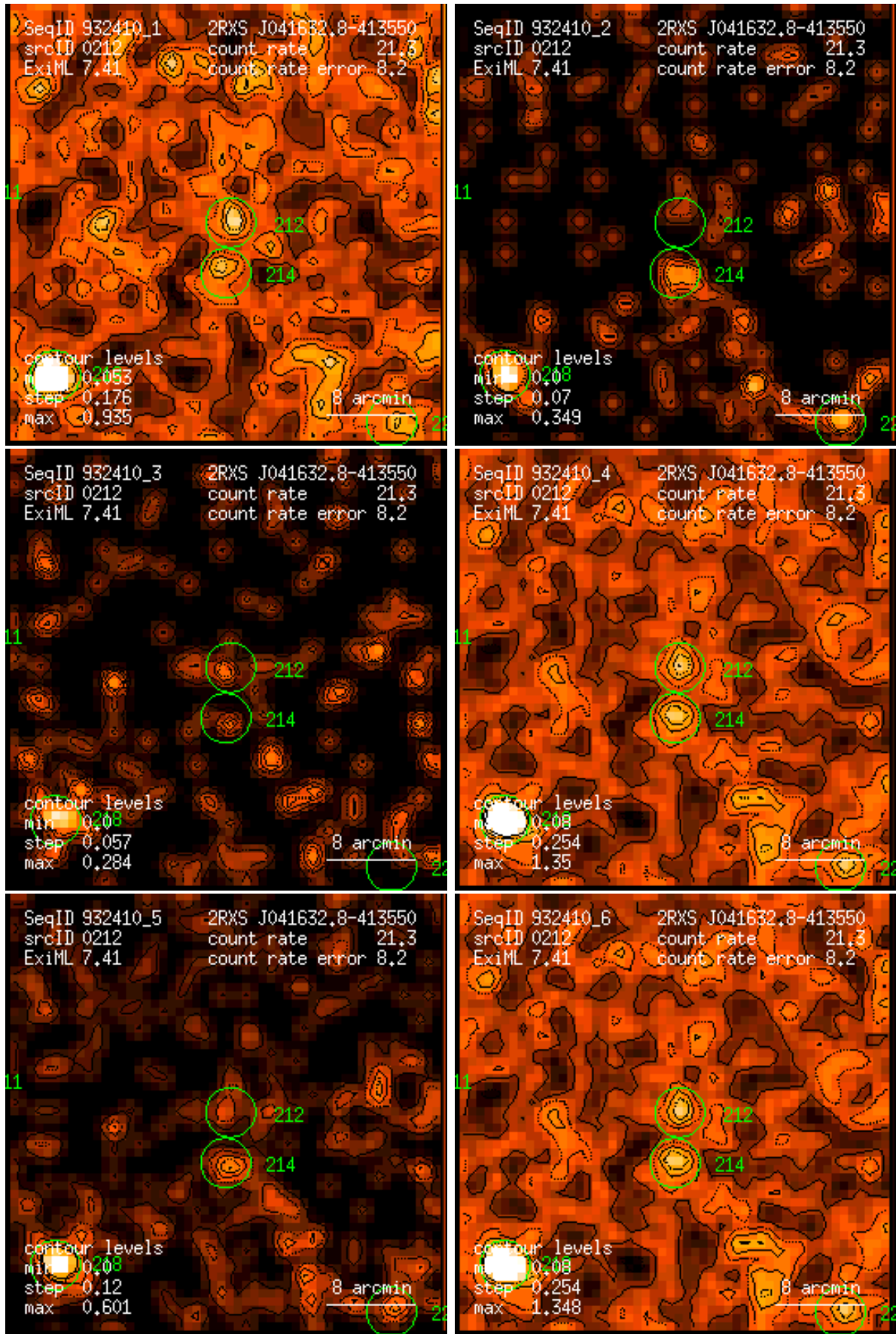
Figure 212: RASS 932410: detection 0212: band rate images, Gaussian filter: (1) PSPC channels 11 – 41, (2) 52 – 90, (3) 91 – 201, (4) 11 – 235, (5) 52 – 201, (6) 11 – 201. Broad band rates in counts/ks. Band rate contour levels in counts/ks/arcmin 2 .
