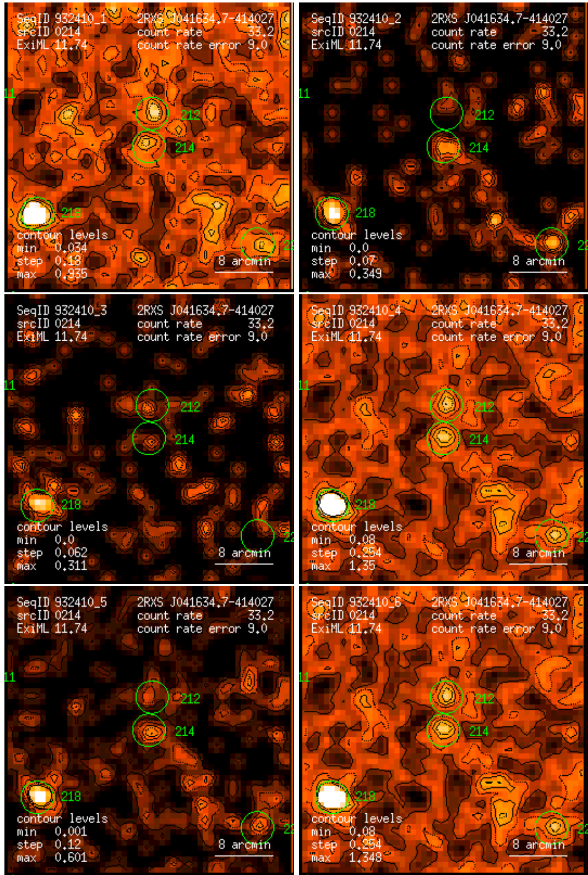
Figure 214: RASS 932410: detection 0214: band rate images, Gaussian filter: (1) PSPC channels 11 – 41, (2) 52 – 90, (3) 91 – 201, (4) 11 – 235, (5) 52 – 201, (6) 11 – 201. Broad band rates in counts/ks. Band rate contour levels in counts/ks/arcmin 2 .
