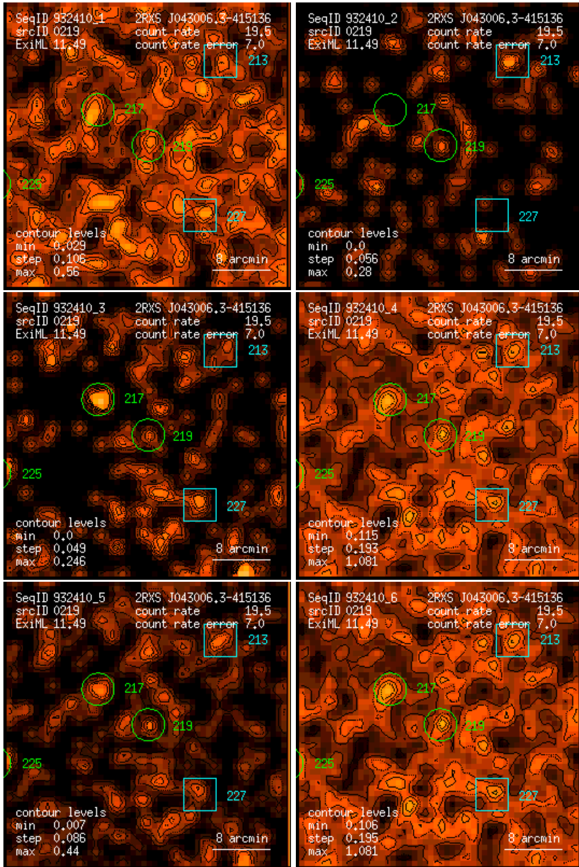
Figure 219: RASS 932410: detection 0219: band rate images, Gaussian filter: (1) PSPC channels 11 – 41, (2) 52 – 90, (3) 91 – 201, (4) 11 – 235, (5) 52 – 201, (6) 11 – 201. Broad band rates in counts/ks. Band rate contour levels in counts/ks/arcmin 2 .
