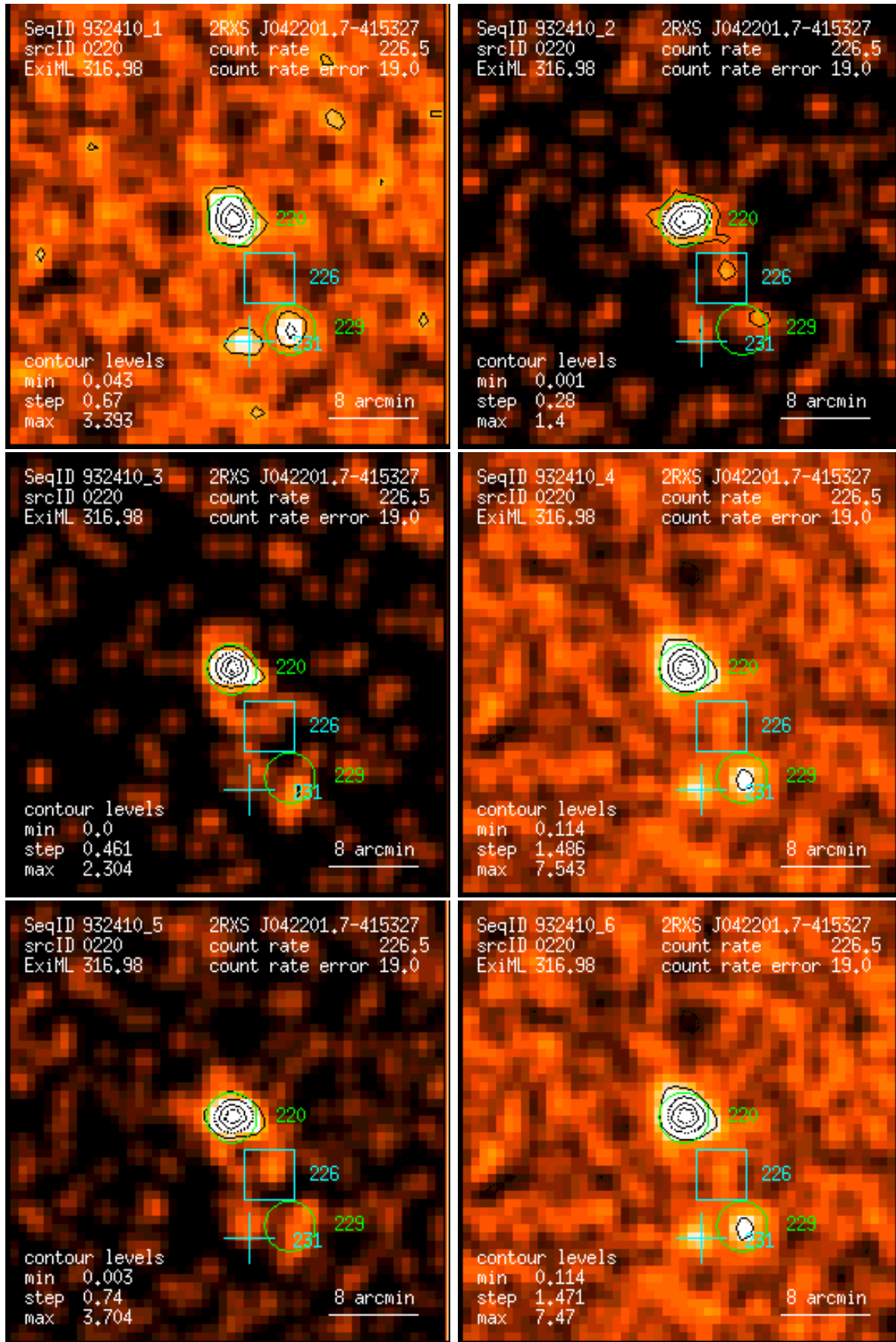
Figure 220: RASS 932410: detection 0220: band rate images, Gaussian filter: (1) PSPC channels 11 – 41, (2) 52 – 90, (3) 91 – 201, (4) 11 – 235, (5) 52 – 201, (6) 11 – 201. Broad band rates in counts/ks. Band rate contour levels in counts/ks/arcmin 2 .
