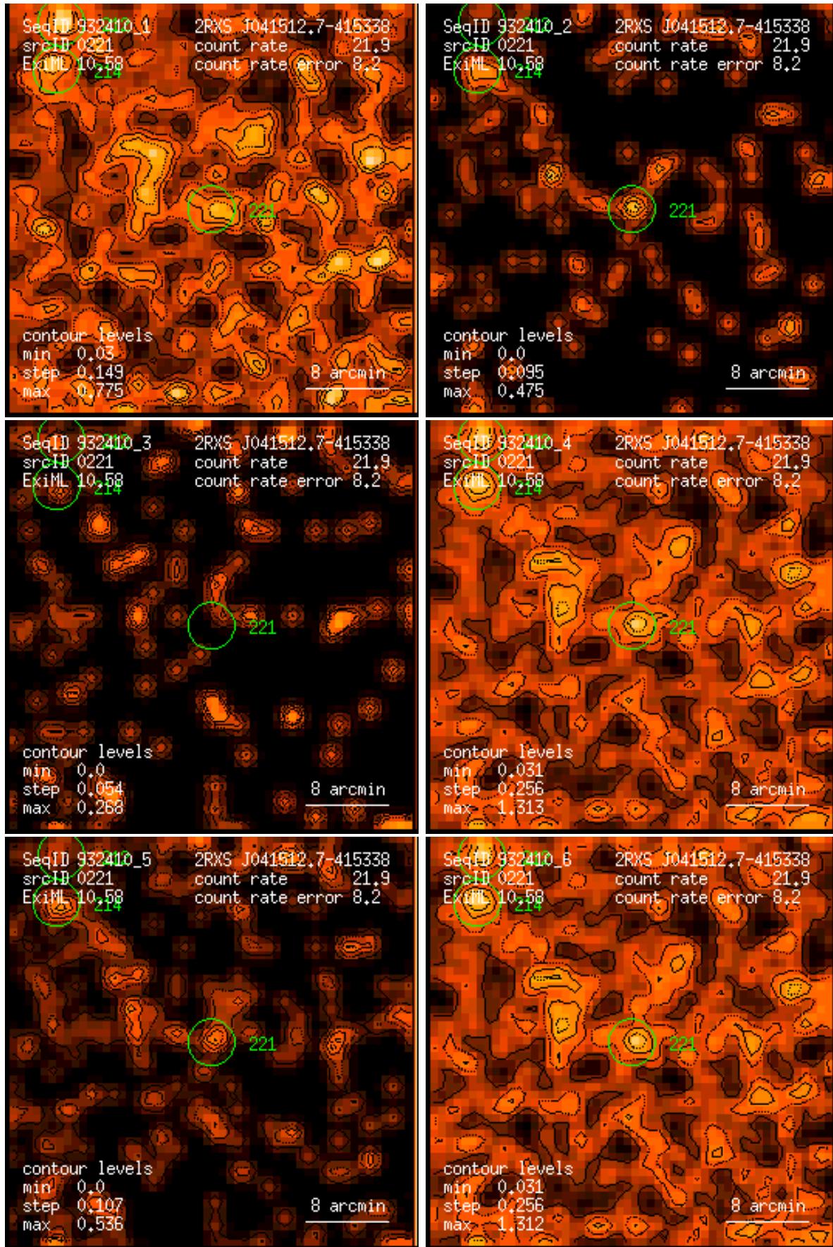
Figure 221: RASS 932410: detection 0221: band rate images, Gaussian filter: (1) PSPC channels 11 – 41, (2) 52 – 90, (3) 91 – 201, (4) 11 – 235, (5) 52 – 201, (6) 11 – 201. Broad band rates in counts/ks. Band rate contour levels in counts/ks/arcmin 2 .
