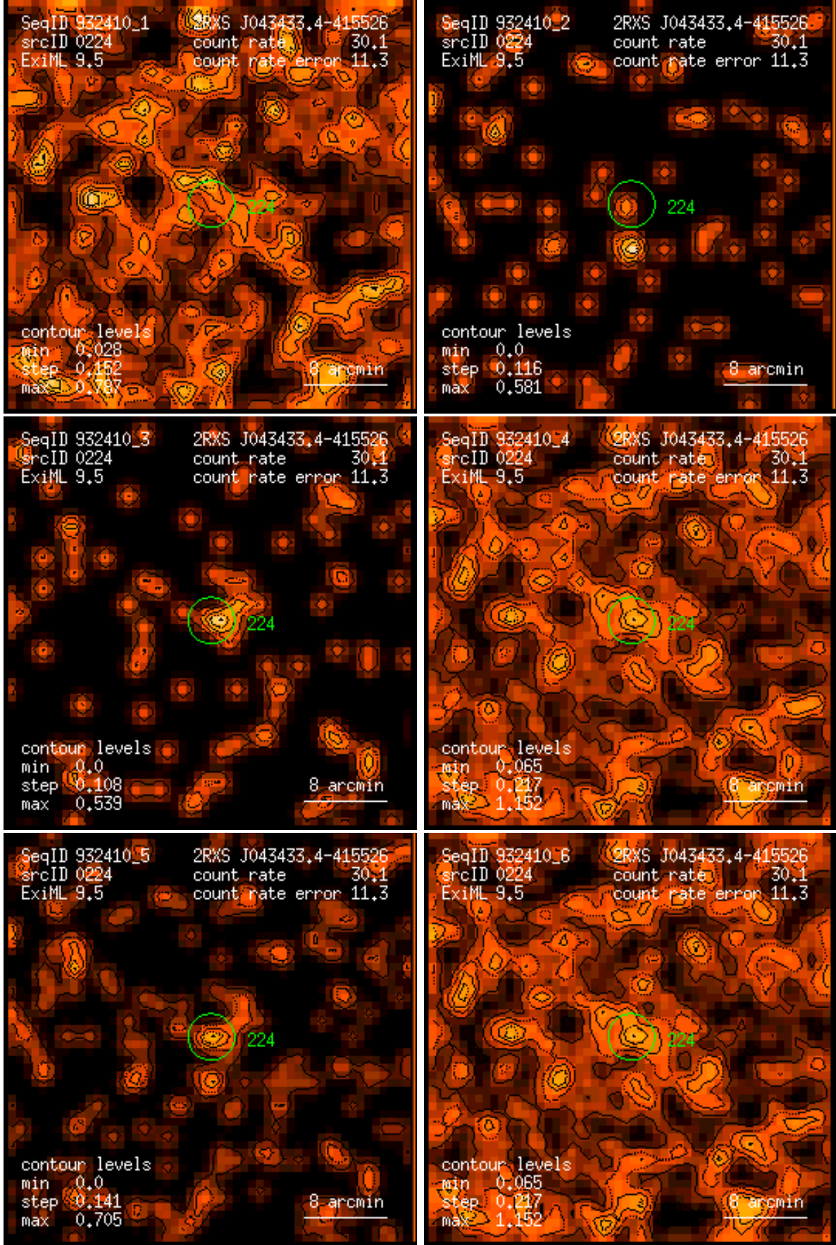
Figure 224: RASS 932410: detection 0224: band rate images, Gaussian filter: (1) PSPC channels 11 – 41, (2) 52 – 90, (3) 91 – 201, (4) 11 – 235, (5) 52 – 201, (6) 11 – 201. Broad band rates in counts/ks. Band rate contour levels in counts/ks/arcmin 2 .
