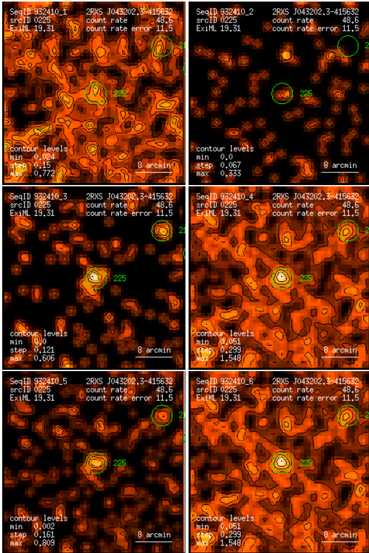
Figure 225: RASS 932410: detection 0225: band rate images, Gaussian filter: (1) PSPC channels 11 – 41, (2) 52 – 90, (3) 91 – 201, (4) 11 – 235, (5) 52 – 201, (6) 11 – 201. Broad band rates in counts/ks. Band rate contour levels in counts/ks/arcmin 2 .
