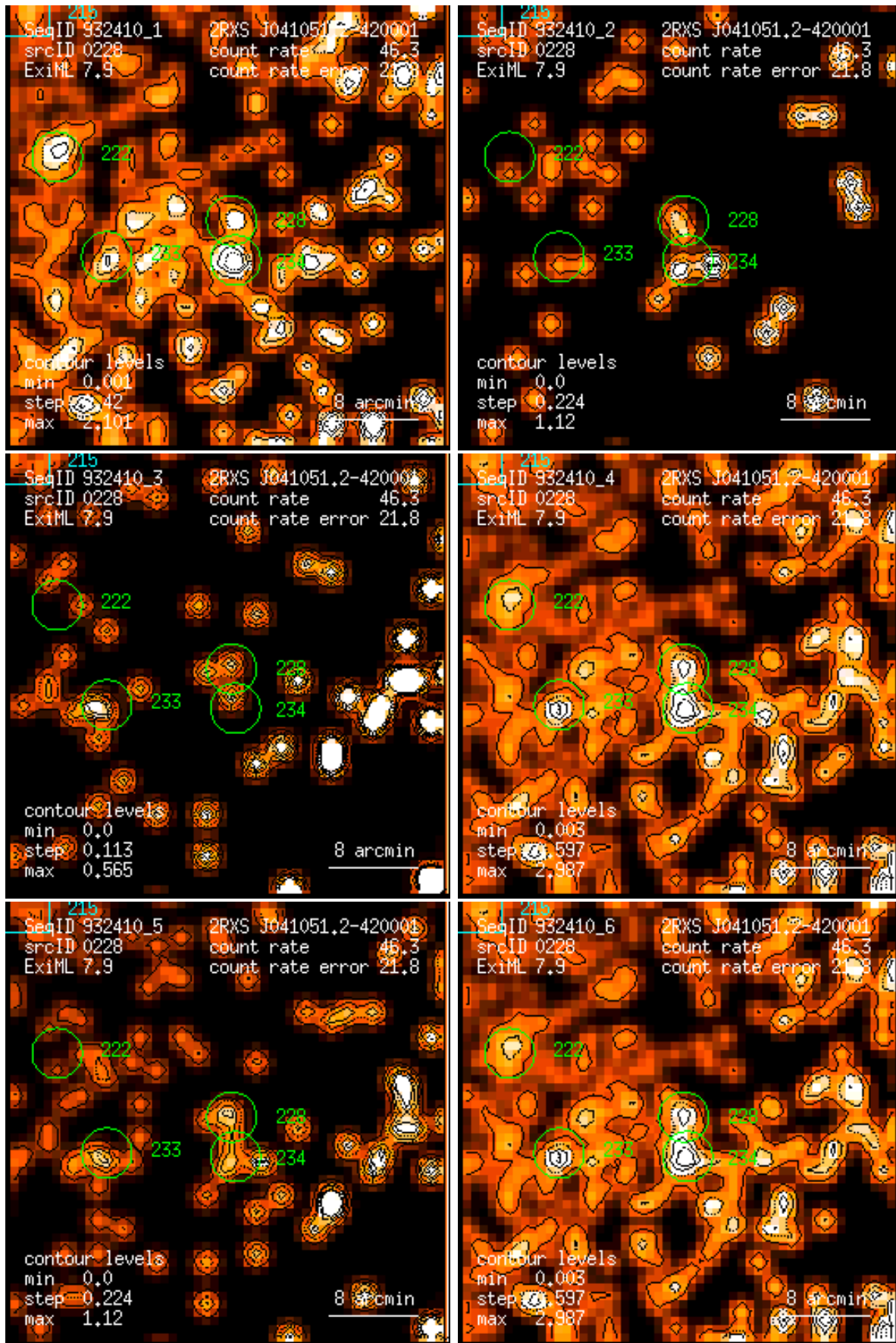
Figure 228: RASS 932410: detection 0228: band rate images, Gaussian filter: (1) PSPC channels 11 – 41, (2) 52 – 90, (3) 91 – 201, (4) 11 – 235, (5) 52 – 201, (6) 11 – 201. Broad band rates in counts/ks. Band rate contour levels in counts/ks/arcmin 2 .
