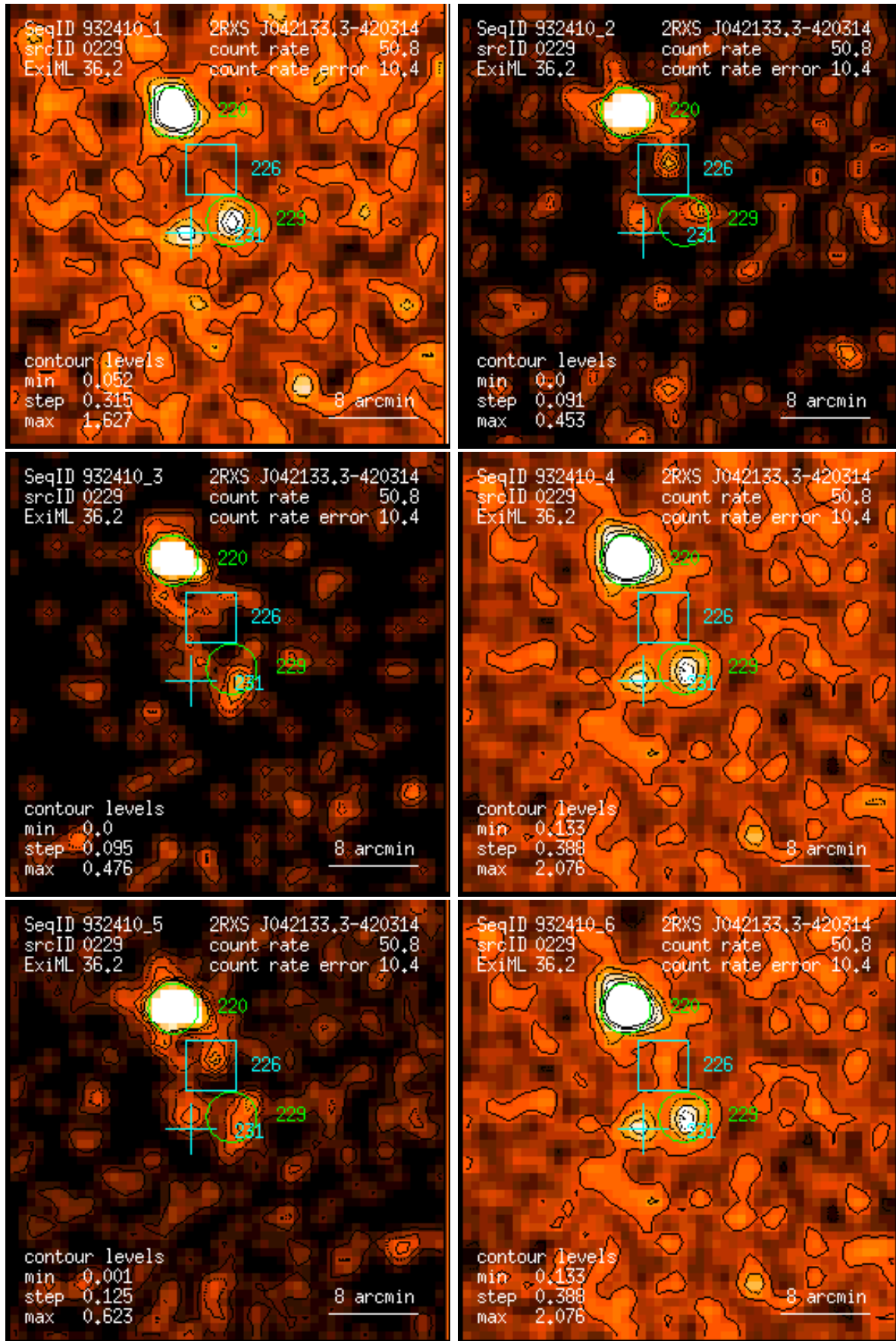
Figure 229: RASS 932410: detection 0229: band rate images, Gaussian filter: (1) PSPC channels 11 – 41, (2) 52 – 90, (3) 91 – 201, (4) 11 – 235, (5) 52 – 201, (6) 11 – 201. Broad band rates in counts/ks. Band rate contour levels in counts/ks/arcmin 2 .
