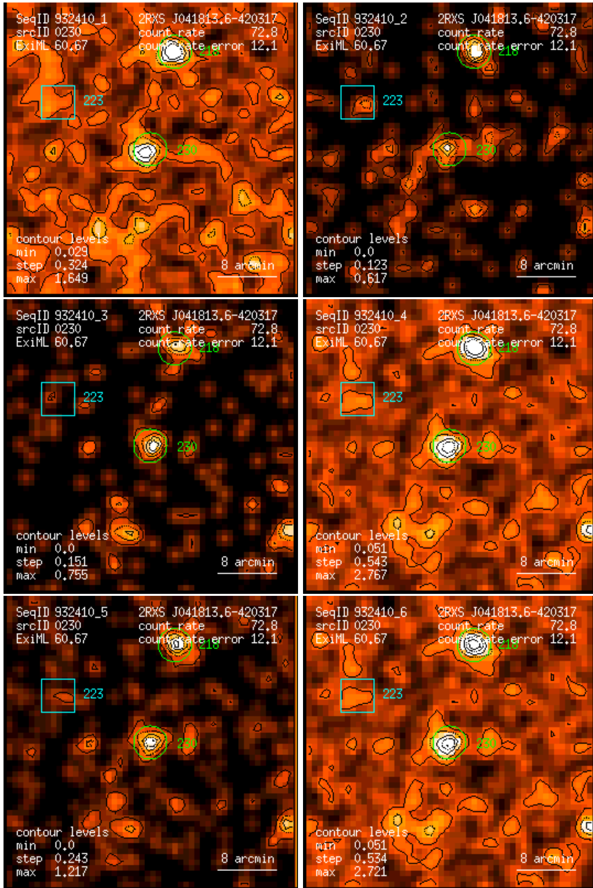
Figure 230: RASS 932410: detection 0230: band rate images, Gaussian filter: (1) PSPC channels 11 – 41, (2) 52 – 90, (3) 91 – 201, (4) 11 – 235, (5) 52 – 201, (6) 11 – 201. Broad band rates in counts/ks. Band rate contour levels in counts/ks/arcmin 2 .
