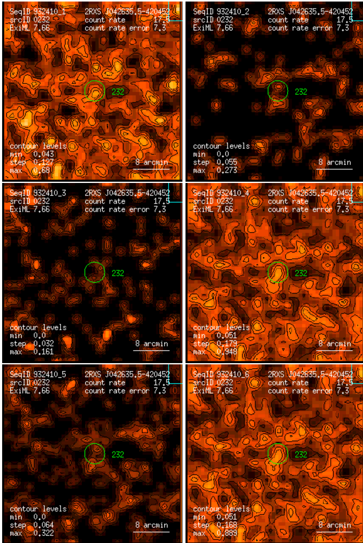
Figure 232: RASS 932410: detection 0232: band rate images, Gaussian filter: (1) PSPC channels 11 – 41, (2) 52 – 90, (3) 91 – 201, (4) 11 – 235, (5) 52 – 201, (6) 11 – 201. Broad band rates in counts/ks. Band rate contour levels in counts/ks/arcmin 2 .
