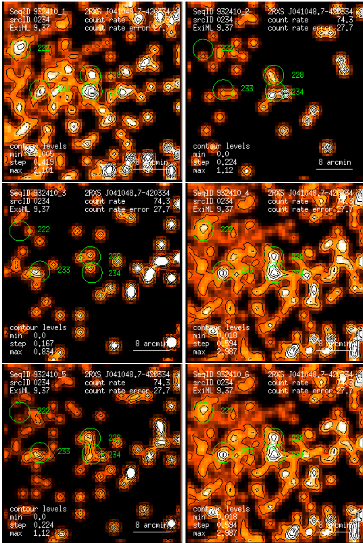
Figure 234: RASS 932410: detection 0234: band rate images, Gaussian filter: (1) PSPC channels 11 – 41, (2) 52 – 90, (3) 91 – 201, (4) 11 – 235, (5) 52 – 201, (6) 11 – 201. Broad band rates in counts/ks. Band rate contour levels in counts/ks/arcmin 2 .
