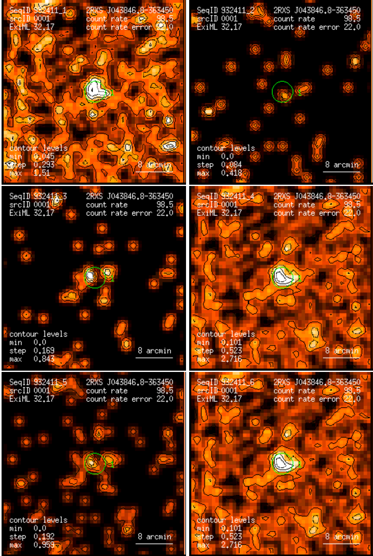
Figure 1: RASS 932411: detection 0001: band rate images, Gaussian filter: (1) PSPC channels 11 – 41, (2) 52 – 90, (3) 91 – 201, (4) 11 – 235, (5) 52 – 201, (6) 11 – 201. Broad band rates in counts/ks. Band rate contour levels in counts/ks/arcmin 2 .
