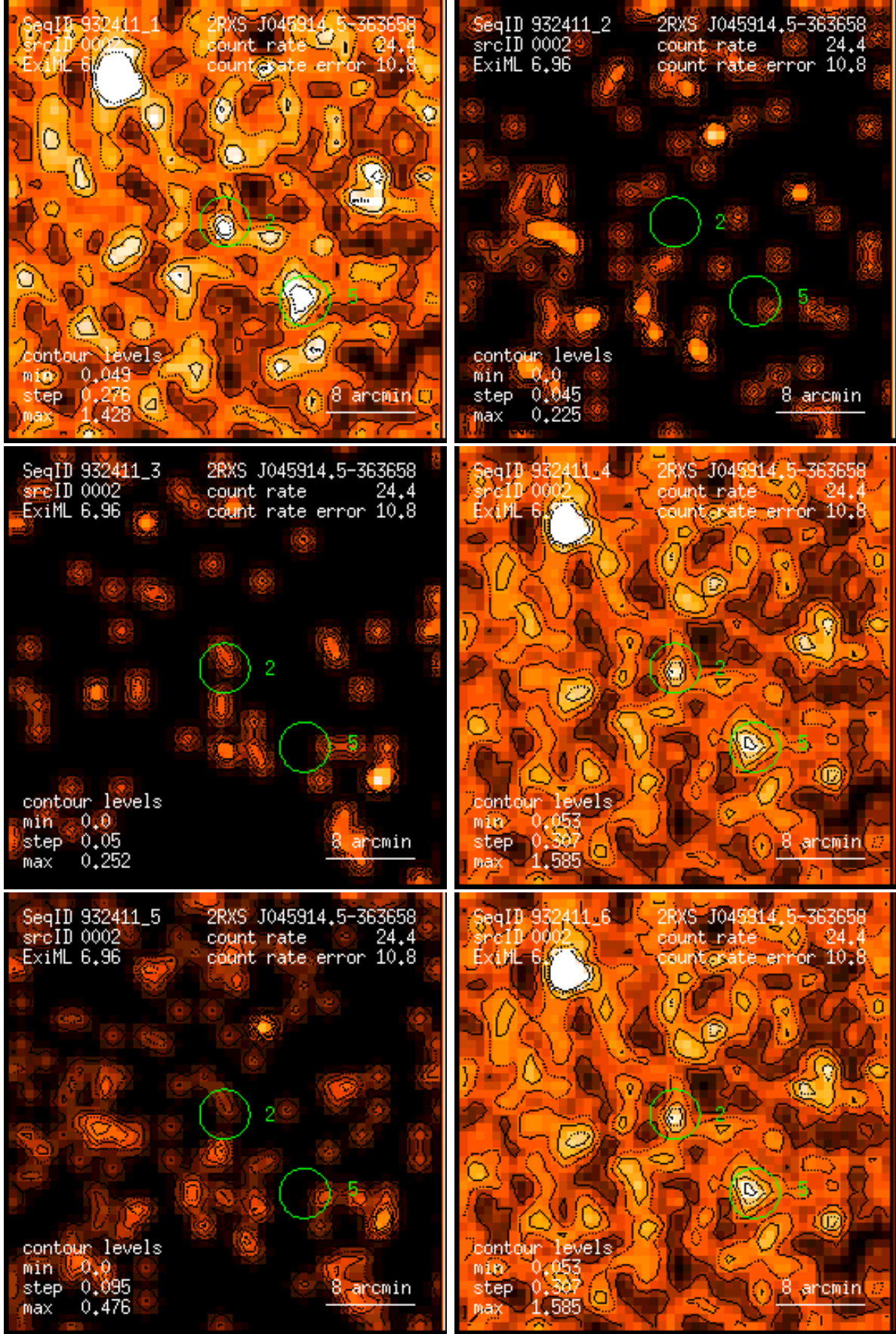
Figure 2: RASS 932411: detection 0002: band rate images, Gaussian filter: (1) PSPC channels 11 – 41, (2) 52 – 90, (3) 91 – 201, (4) 11 – 235, (5) 52 – 201, (6) 11 – 201. Broad band rates in counts/ks. Band rate contour levels in counts/ks/arcmin 2 .
