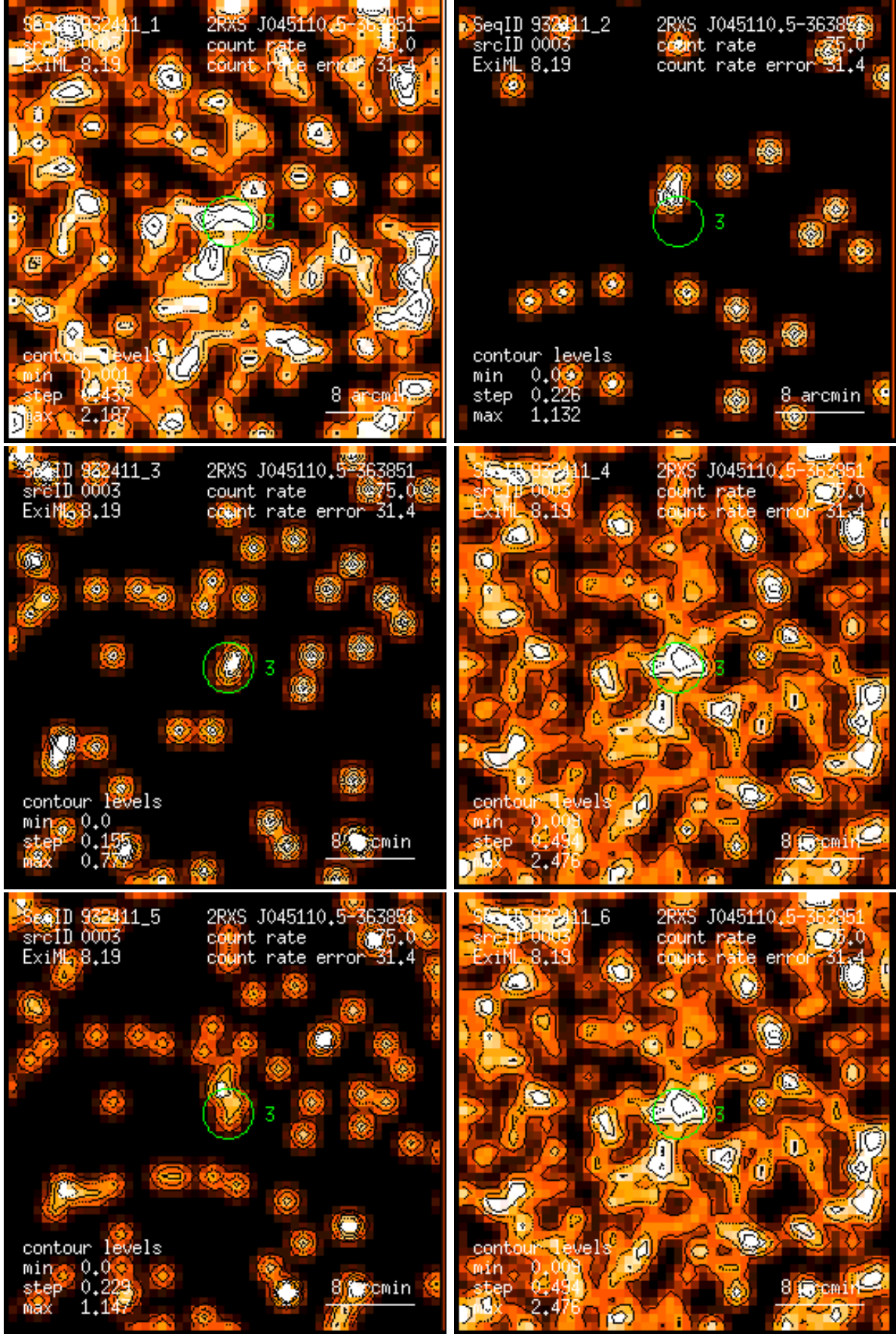
Figure 3: RASS 932411: detection 0003: band rate images, Gaussian filter: (1) PSPC channels 11 – 41, (2) 52 – 90, (3) 91 – 201, (4) 11 – 235, (5) 52 – 201, (6) 11 – 201. Broad band rates in counts/ks. Band rate contour levels in counts/ks/arcmin 2 .
