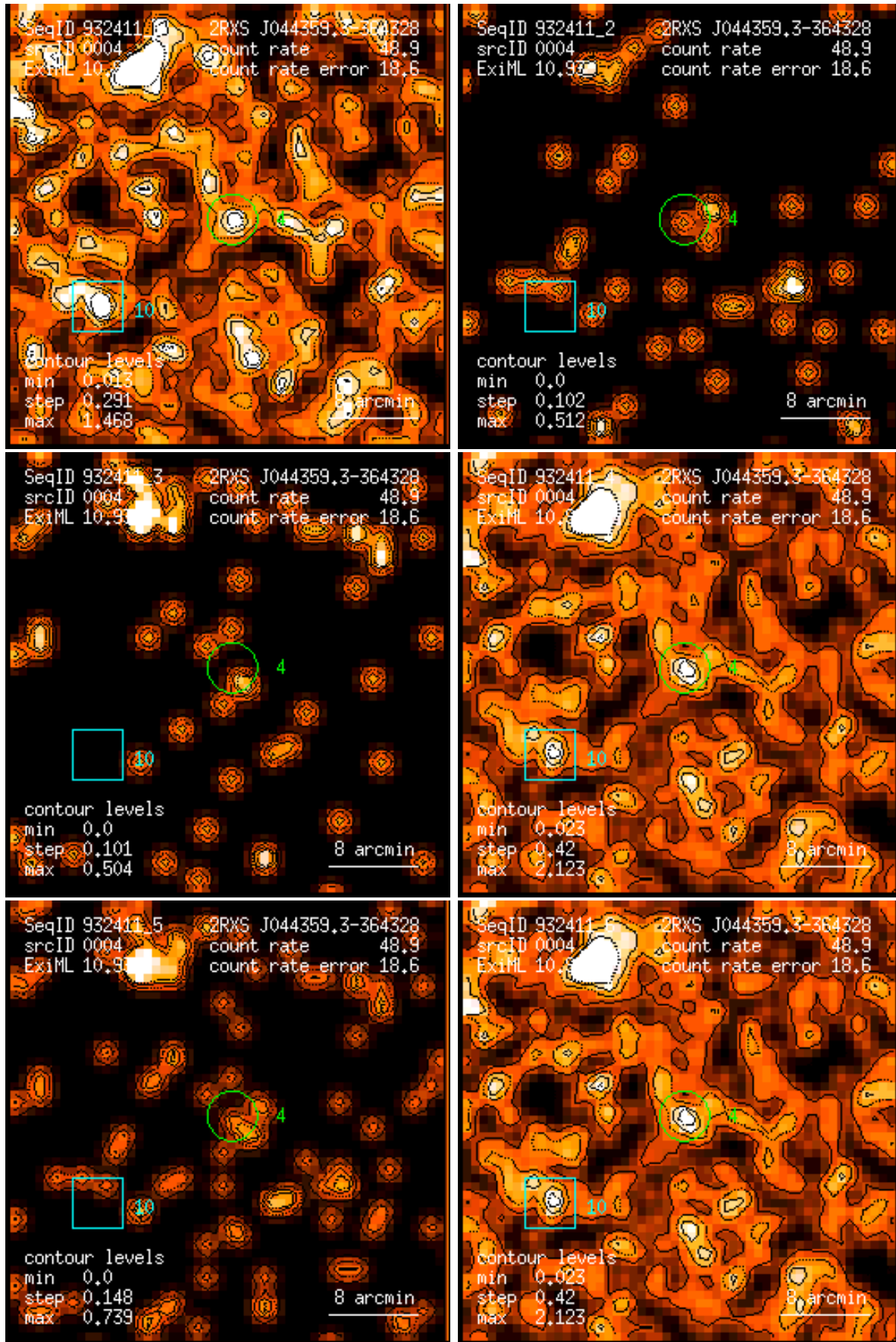
Figure 4: RASS 932411: detection 0004: band rate images, Gaussian filter: (1) PSPC channels 11 – 41, (2) 52 – 90, (3) 91 – 201, (4) 11 – 235, (5) 52 – 201, (6) 11 – 201. Broad band rates in counts/ks. Band rate contour levels in counts/ks/arcmin 2 .
