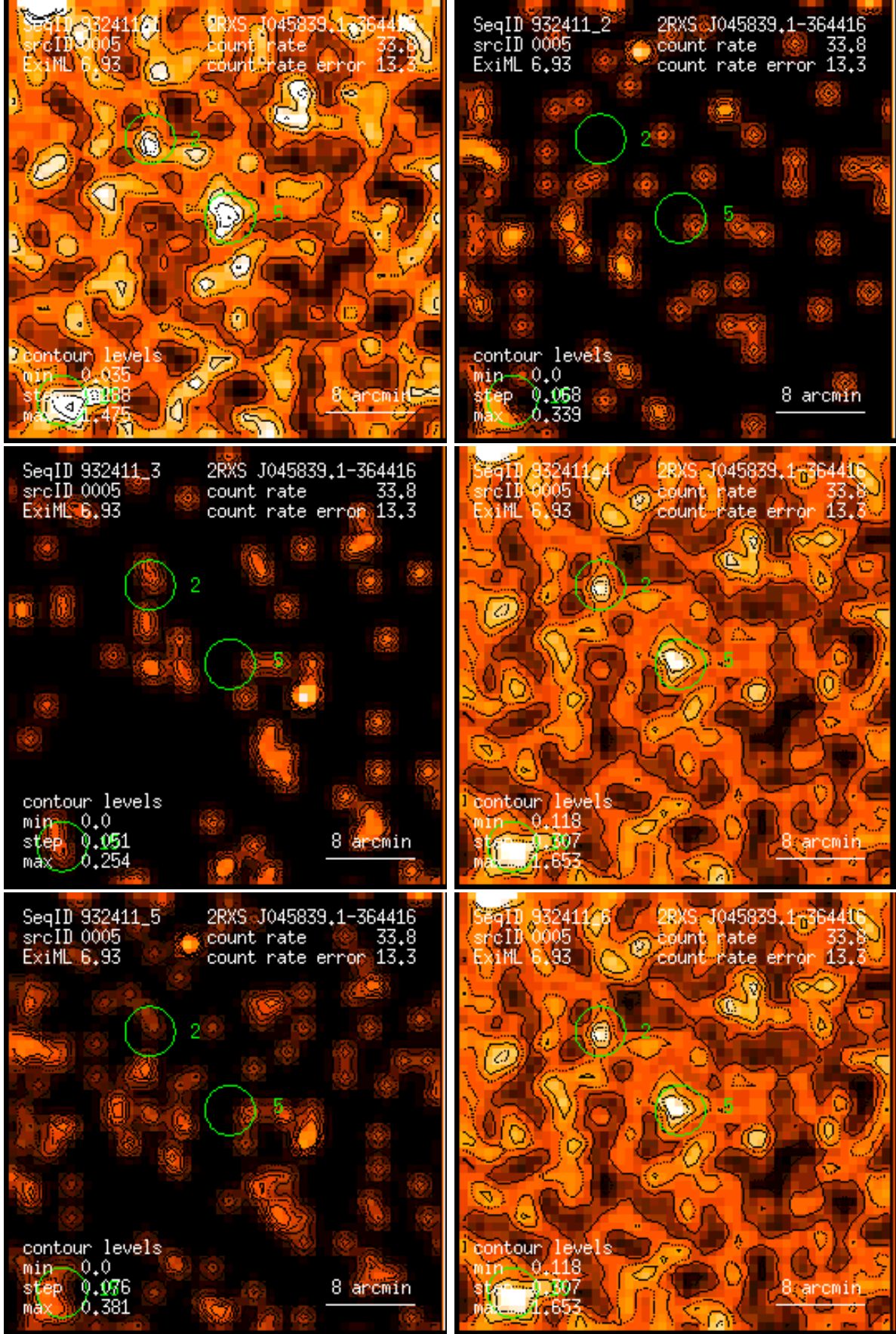
Figure 5: RASS 932411: detection 0005: band rate images, Gaussian filter: (1) PSPC channels 11 – 41, (2) 52 – 90, (3) 91 – 201, (4) 11 – 235, (5) 52 – 201, (6) 11 – 201. Broad band rates in counts/ks. Band rate contour levels in counts/ks/arcmin 2 .
