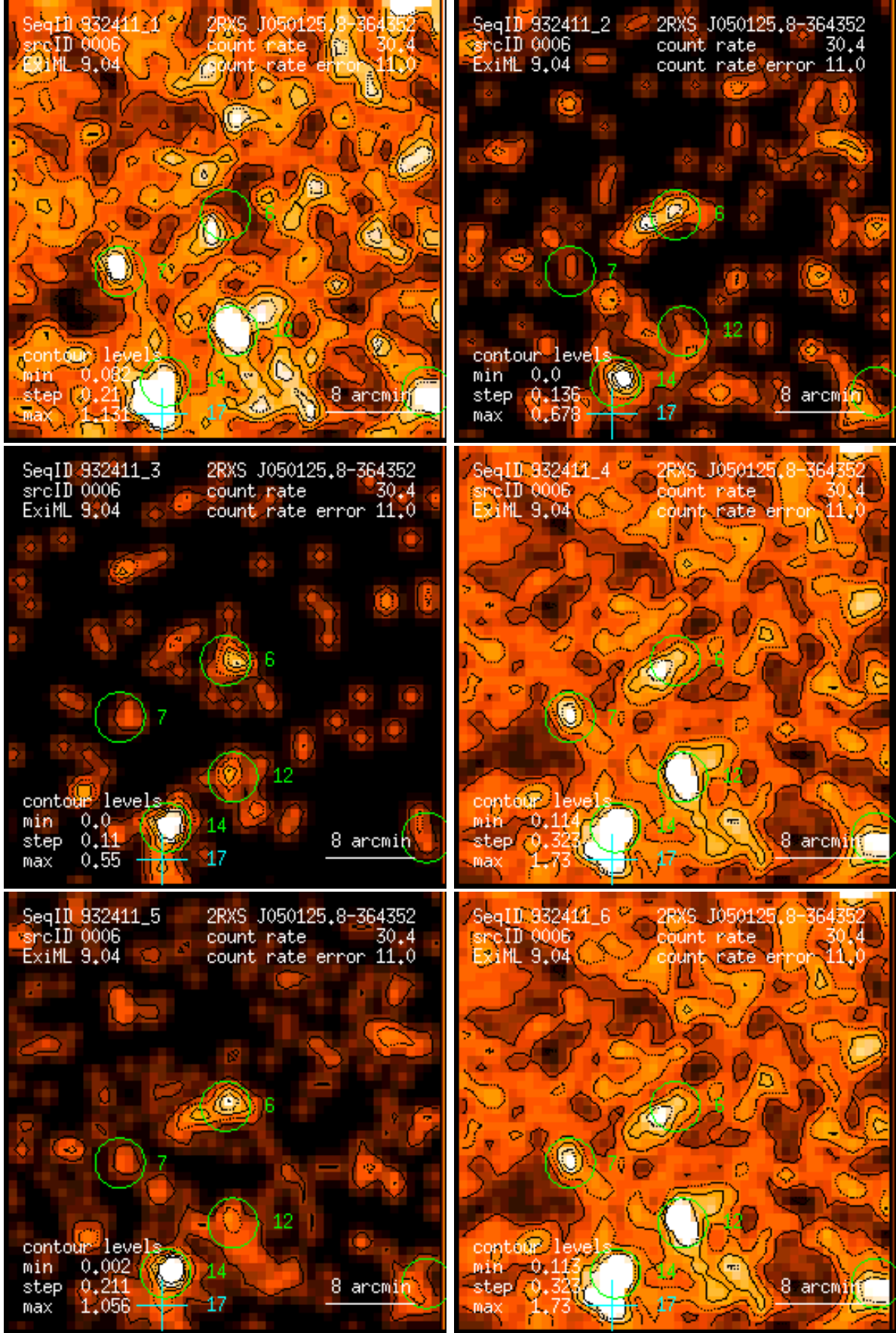
Figure 6: RASS 932411: detection 0006: band rate images, Gaussian filter: (1) PSPC channels 11 – 41, (2) 52 – 90, (3) 91 – 201, (4) 11 – 235, (5) 52 – 201, (6) 11 – 201. Broad band rates in counts/ks. Band rate contour levels in counts/ks/arcmin 2 .
