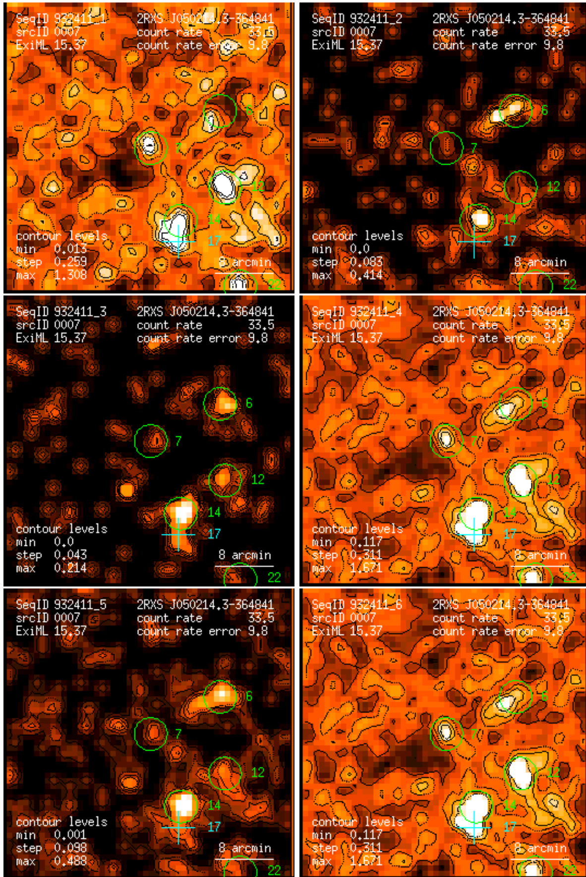
Figure 7: RASS 932411: detection 0007: band rate images, Gaussian filter: (1) PSPC channels 11 – 41, (2) 52 – 90, (3) 91 – 201, (4) 11 – 235, (5) 52 – 201, (6) 11 – 201. Broad band rates in counts/ks. Band rate contour levels in counts/ks/arcmin 2 .
