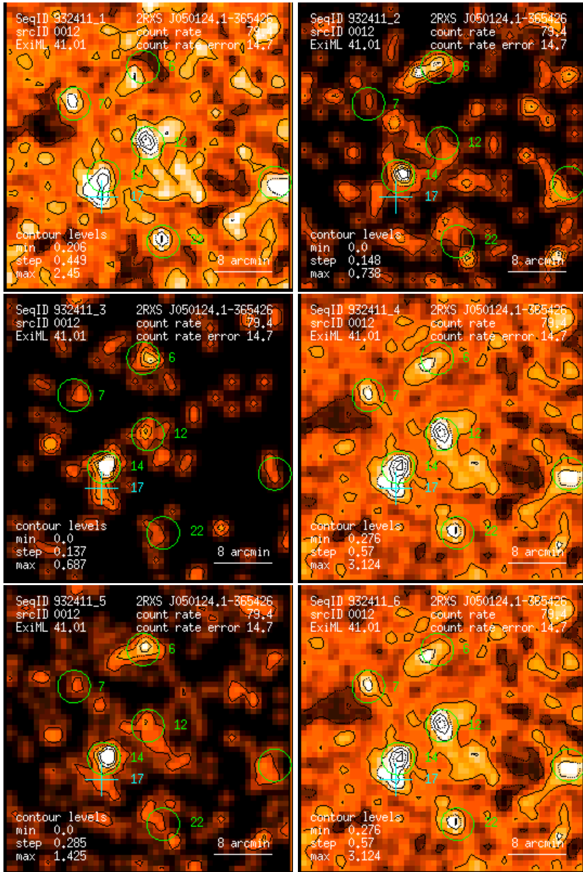
Figure 12: RASS 932411: detection 0012: band rate images, Gaussian filter: (1) PSPC channels 11 – 41, (2) 52 – 90, (3) 91 – 201, (4) 11 – 235, (5) 52 – 201, (6) 11 – 201. Broad band rates in counts/ks. Band rate contour levels in counts/ks/arcmin 2 .
