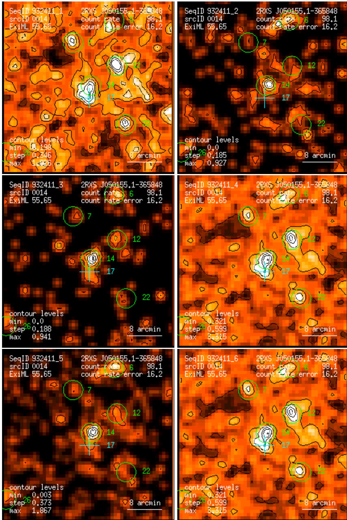
Figure 14: RASS 932411: detection 0014: band rate images, Gaussian filter: (1) PSPC channels 11 – 41, (2) 52 – 90, (3) 91 – 201, (4) 11 – 235, (5) 52 – 201, (6) 11 – 201. Broad band rates in counts/ks. Band rate contour levels in counts/ks/arcmin 2 .
