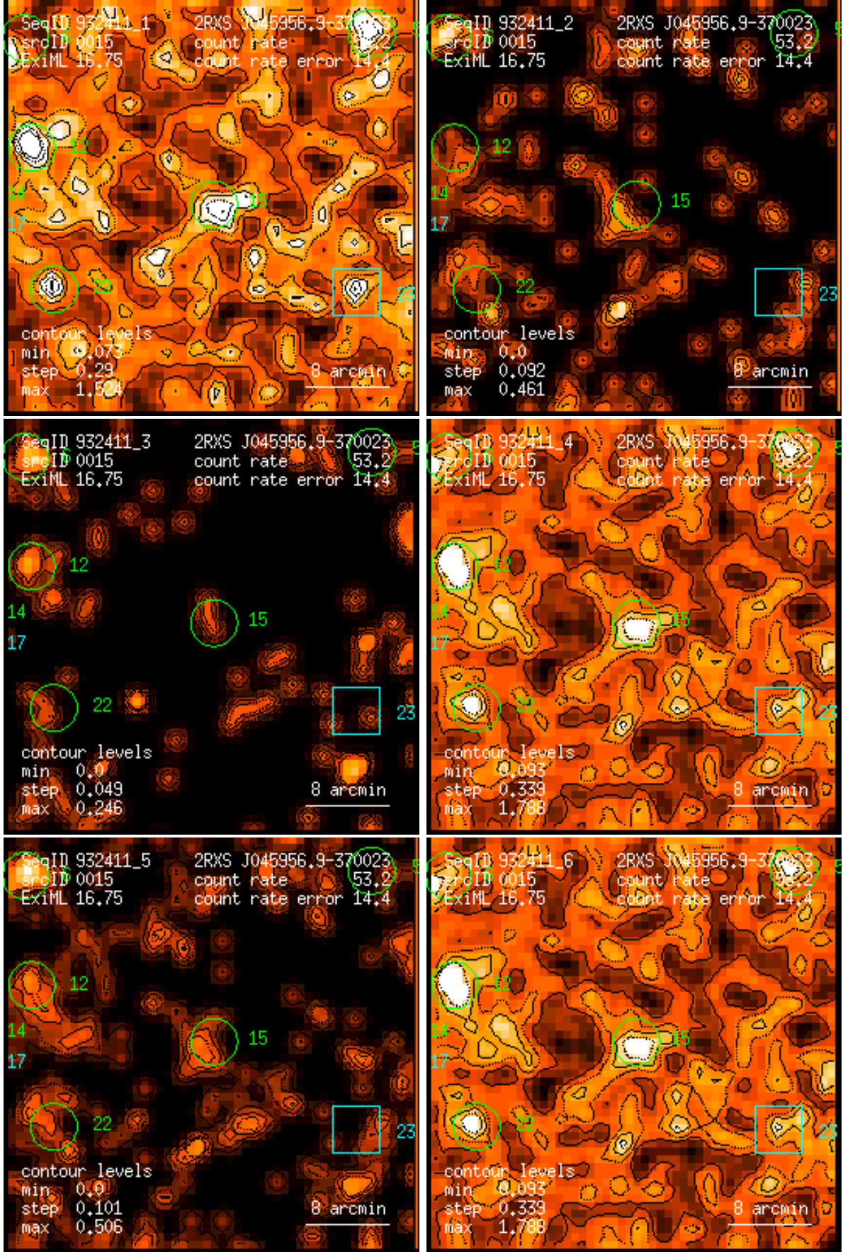
Figure 15: RASS 932411: detection 0015: band rate images, Gaussian filter: (1) PSPC channels 11 – 41, (2) 52 – 90, (3) 91 – 201, (4) 11 – 235, (5) 52 – 201, (6) 11 – 201. Broad band rates in counts/ks. Band rate contour levels in counts/ks/arcmin 2 .
