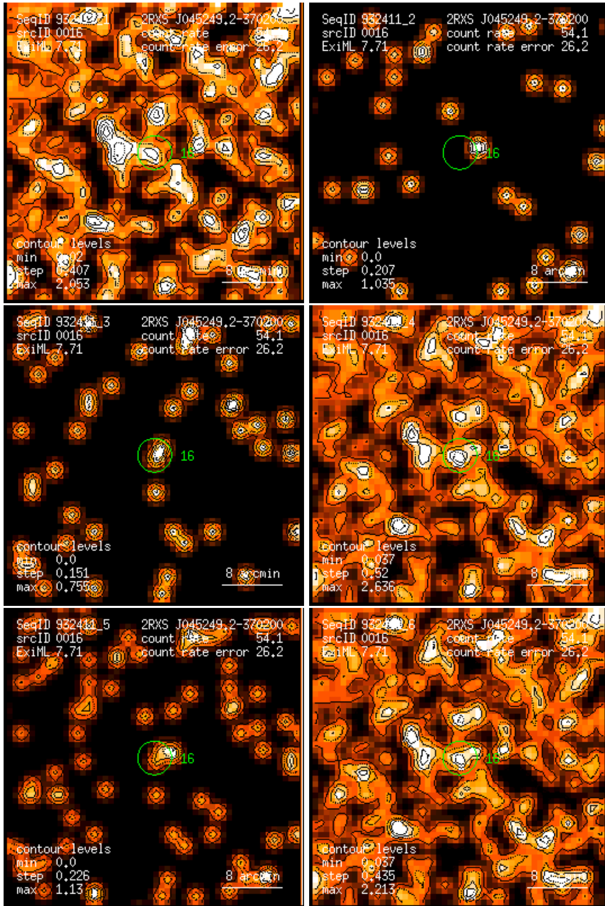
Figure 16: RASS 932411: detection 0016: band rate images, Gaussian filter: (1) PSPC channels 11 – 41, (2) 52 – 90, (3) 91 – 201, (4) 11 – 235, (5) 52 – 201, (6) 11 – 201. Broad band rates in counts/ks. Band rate contour levels in counts/ks/arcmin 2 .
