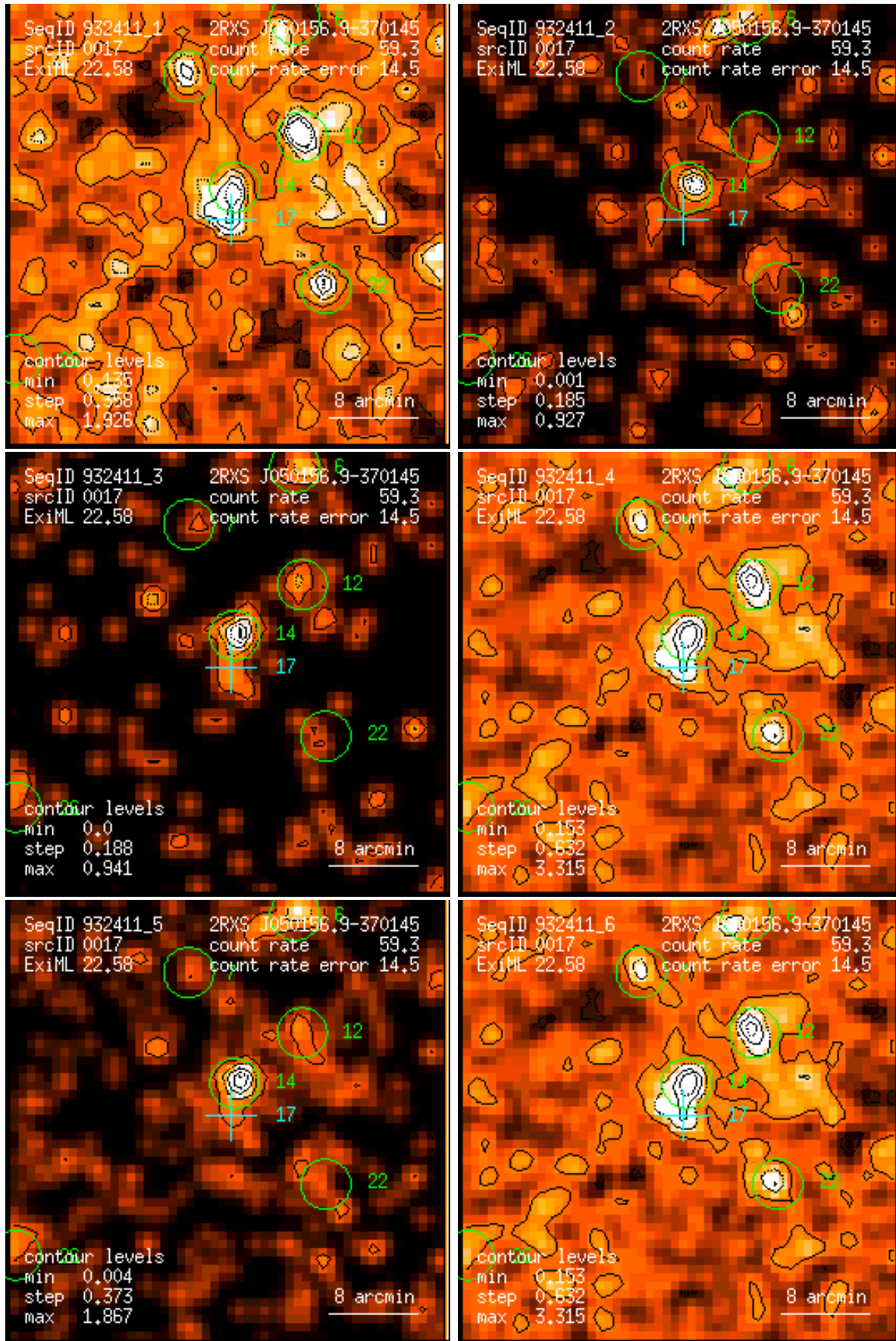
Figure 17: RASS 932411: detection 0017: band rate images, Gaussian filter: (1) PSPC channels 11 – 41, (2) 52 – 90, (3) 91 – 201, (4) 11 – 235, (5) 52 – 201, (6) 11 – 201. Broad band rates in counts/ks. Band rate contour levels in counts/ks/arcmin 2 .
