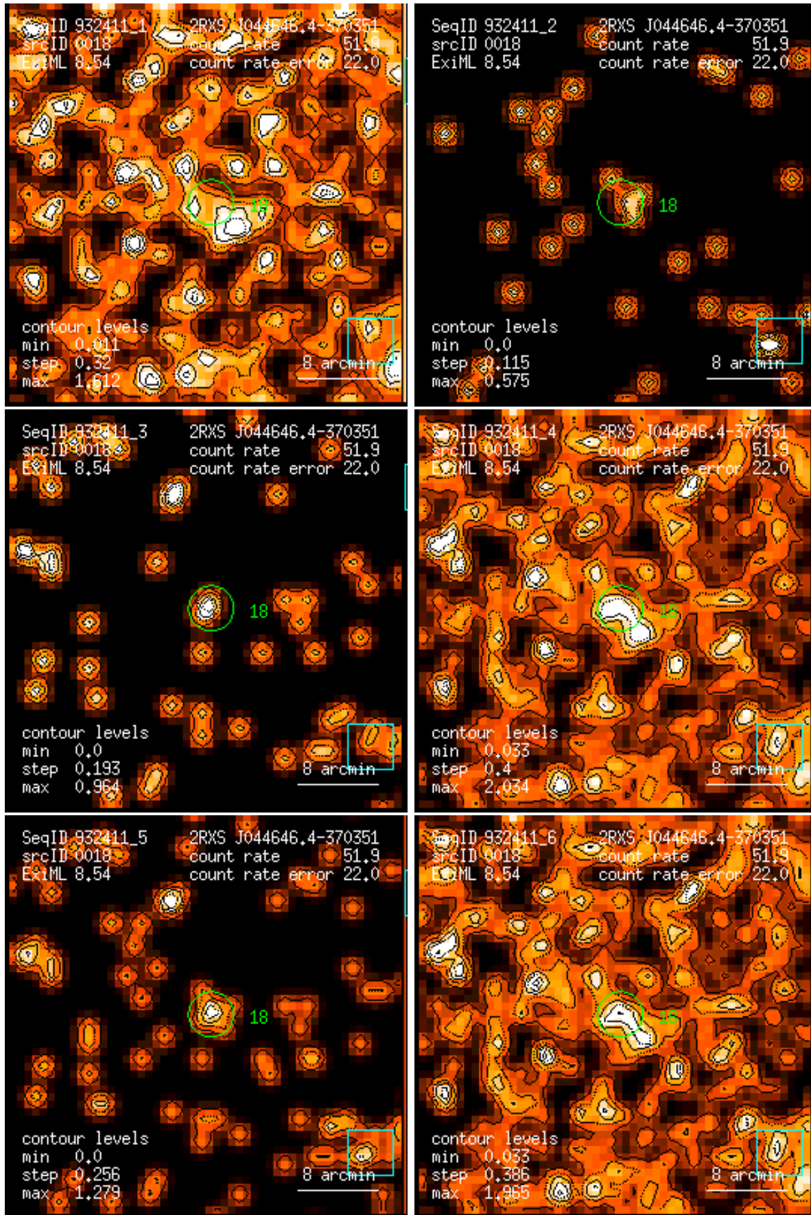
Figure 18: RASS 932411: detection 0018: band rate images, Gaussian filter: (1) PSPC channels 11 – 41, (2) 52 – 90, (3) 91 – 201, (4) 11 – 235, (5) 52 – 201, (6) 11 – 201. Broad band rates in counts/ks. Band rate contour levels in counts/ks/arcmin 2 .
