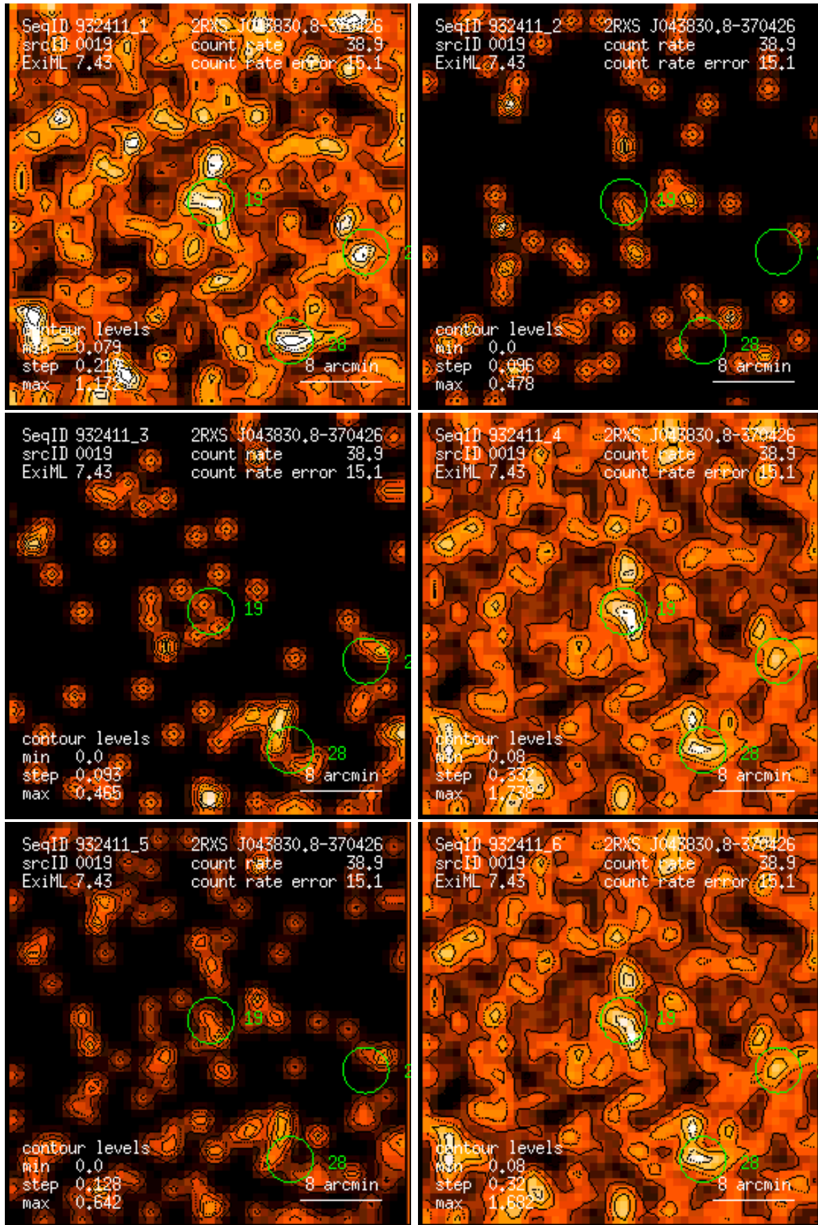
Figure 19: RASS 932411: detection 0019: band rate images, Gaussian filter: (1) PSPC channels 11 – 41, (2) 52 – 90, (3) 91 – 201, (4) 11 – 235, (5) 52 – 201, (6) 11 – 201. Broad band rates in counts/ks. Band rate contour levels in counts/ks/arcmin 2 .
